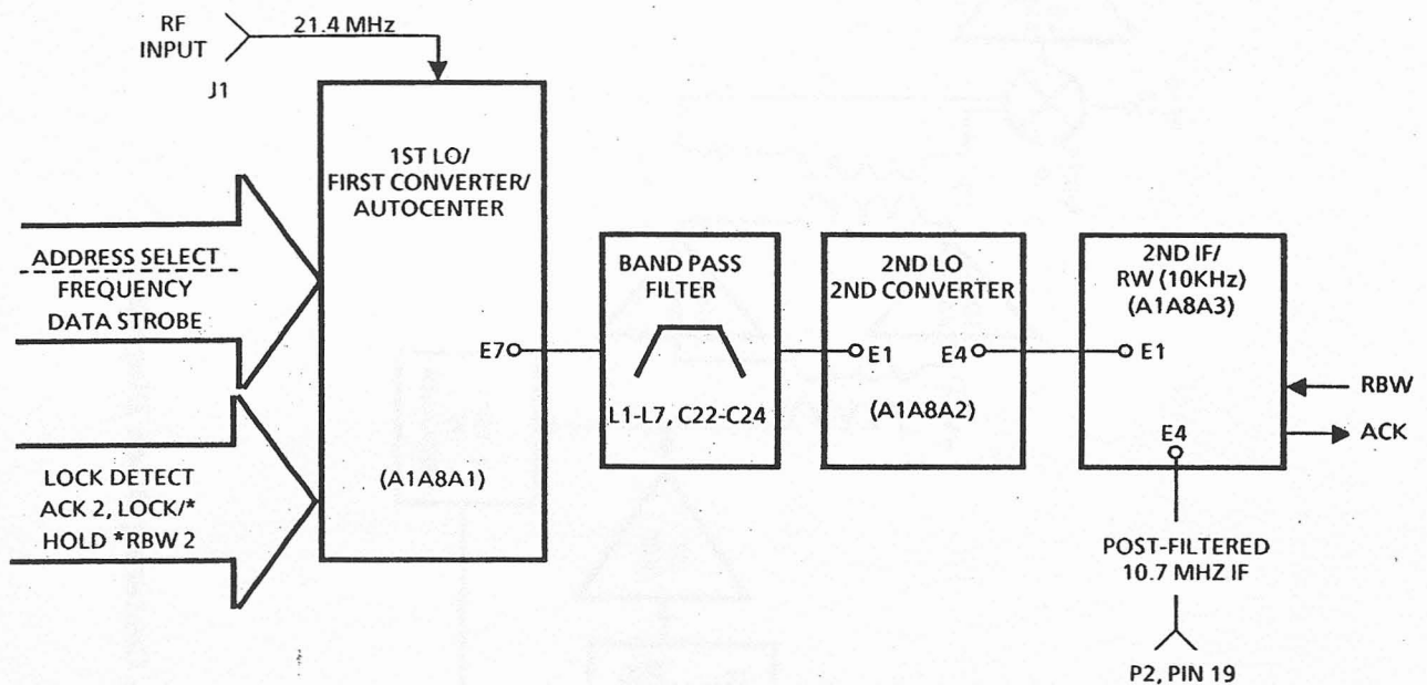
Figure 3-9. Frequency Converter/Sweep Assembly Block Diagram
