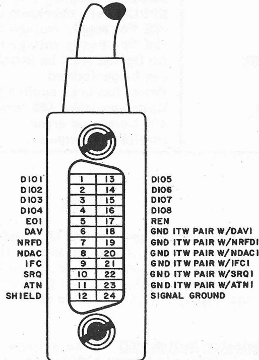
Figure 2-5. Configuration of IEEE-488 Data Bus
