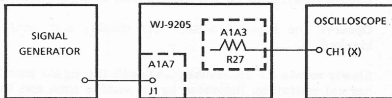
Figure 4-4. DRD/Timing Control Alignment, Equipment Connections
