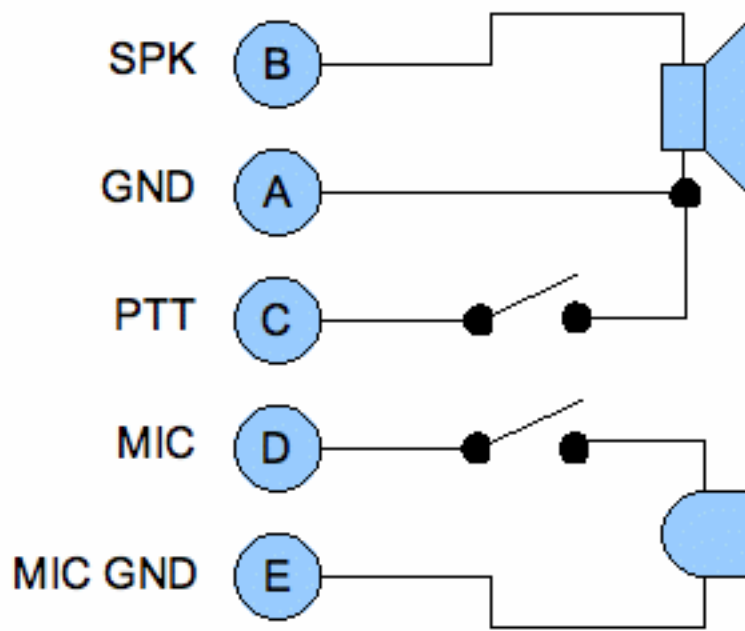
H-356 Handset
