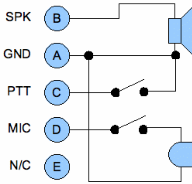
H-250 Handset
