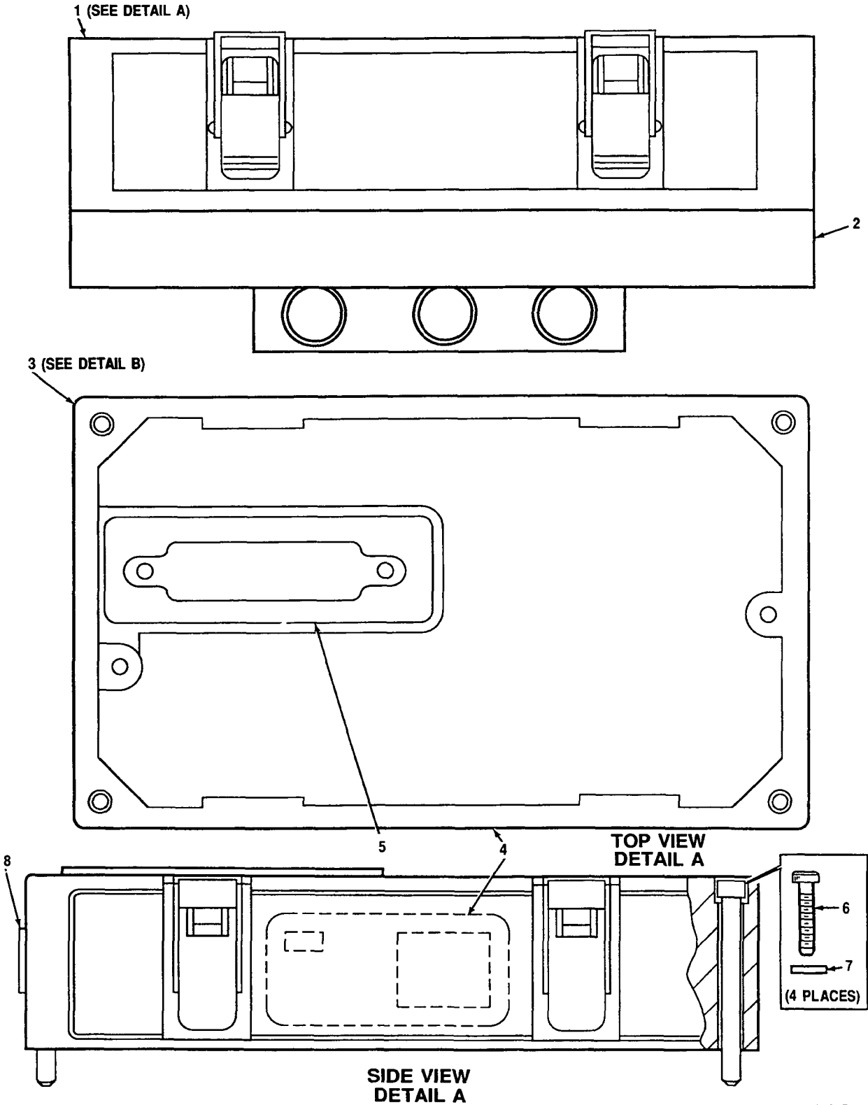
Figure 14. tone Converter A2A1 (A3026047) (Sheet 1 of 2)
