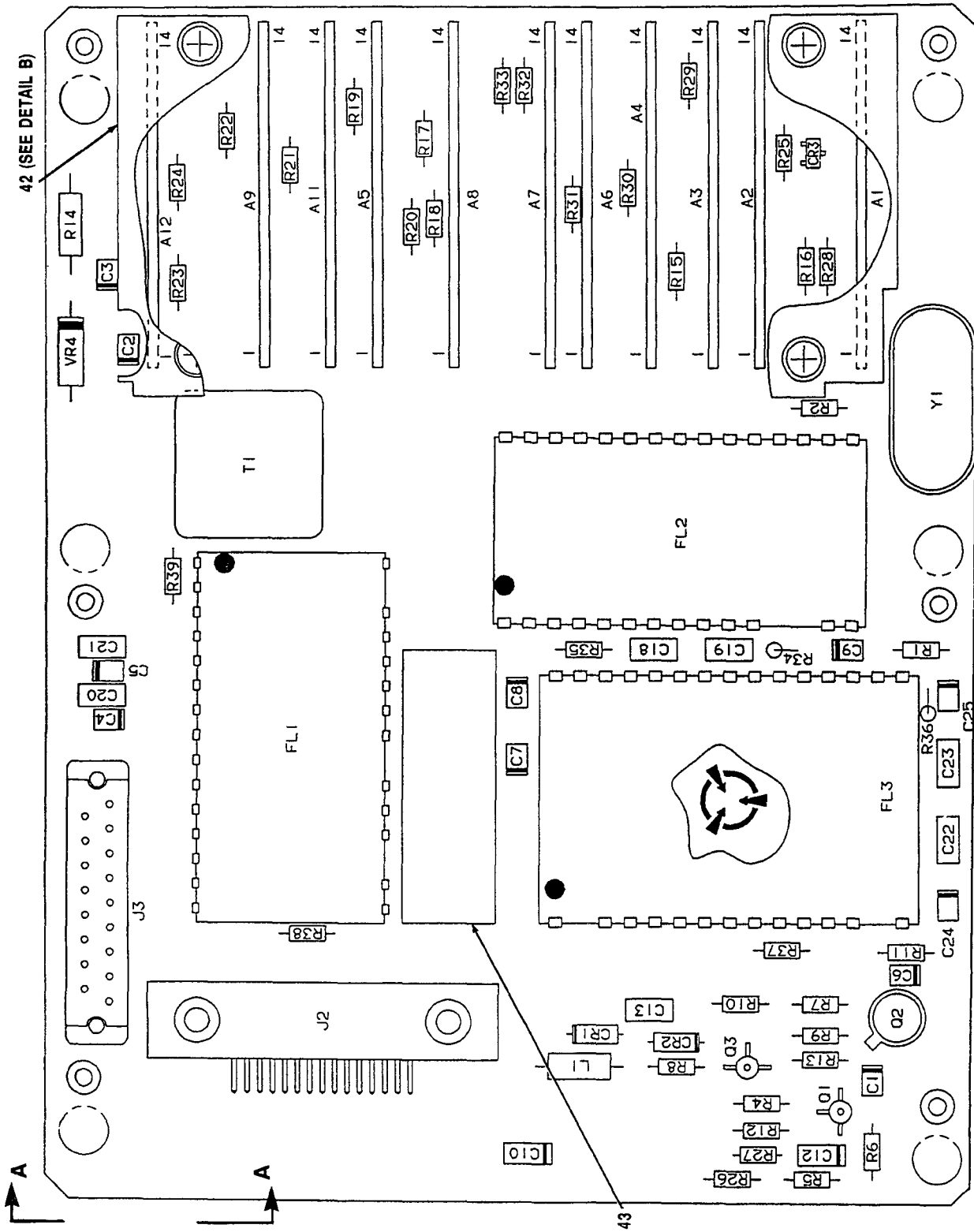
Figure 8. Circuit Card Assembly A1A1A2 (A3027437) (Sheet 1 of 2)
