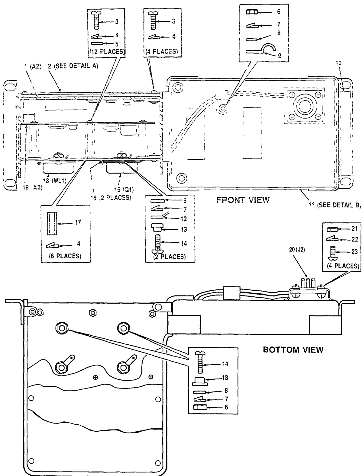
Figure 7 RCS Remote Chassis (A3030432) (Sheet 1 of 2)
