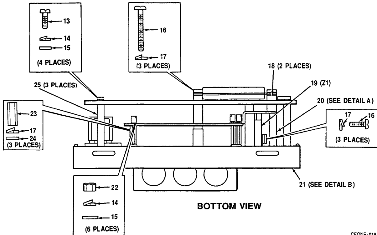
Figure 15. Front Tone converter Assembly (A3030366) (Sheet 1 of 5)
