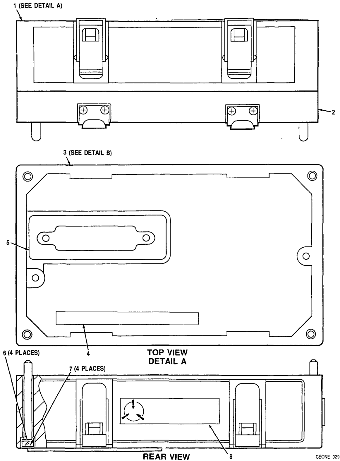
Figure 19. DC/DC Converter A2A2 (A3026048) (Sheet 1 of 2)
