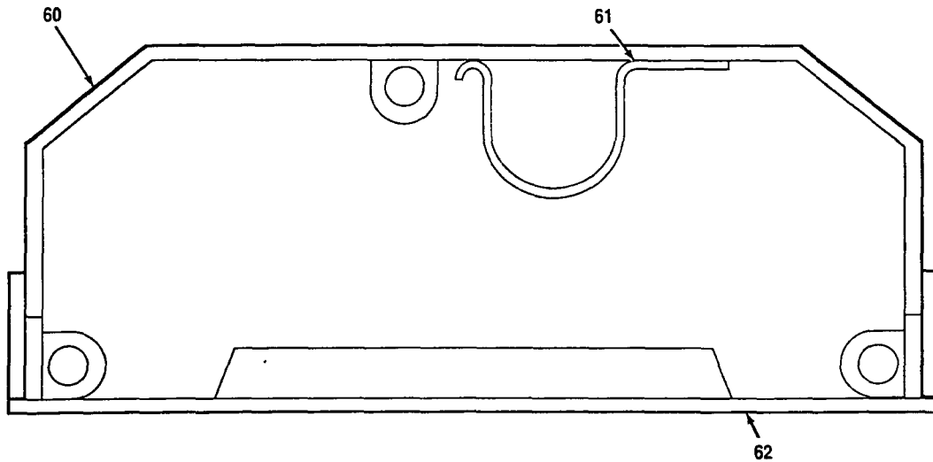
DETAIL D
