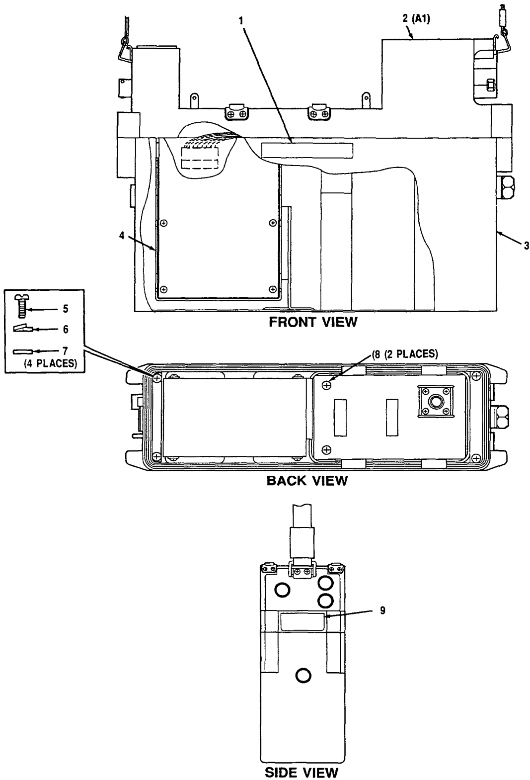
Figure 3. Converter, Keyer A1A1 (A3026045)
