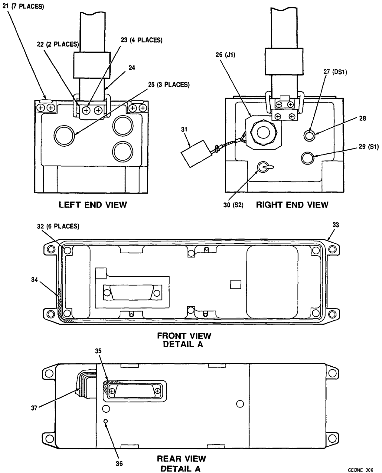
Figure 5. Front Panel Assembly A1A1A1 (A3030434) (Sheet 2 of 2)
