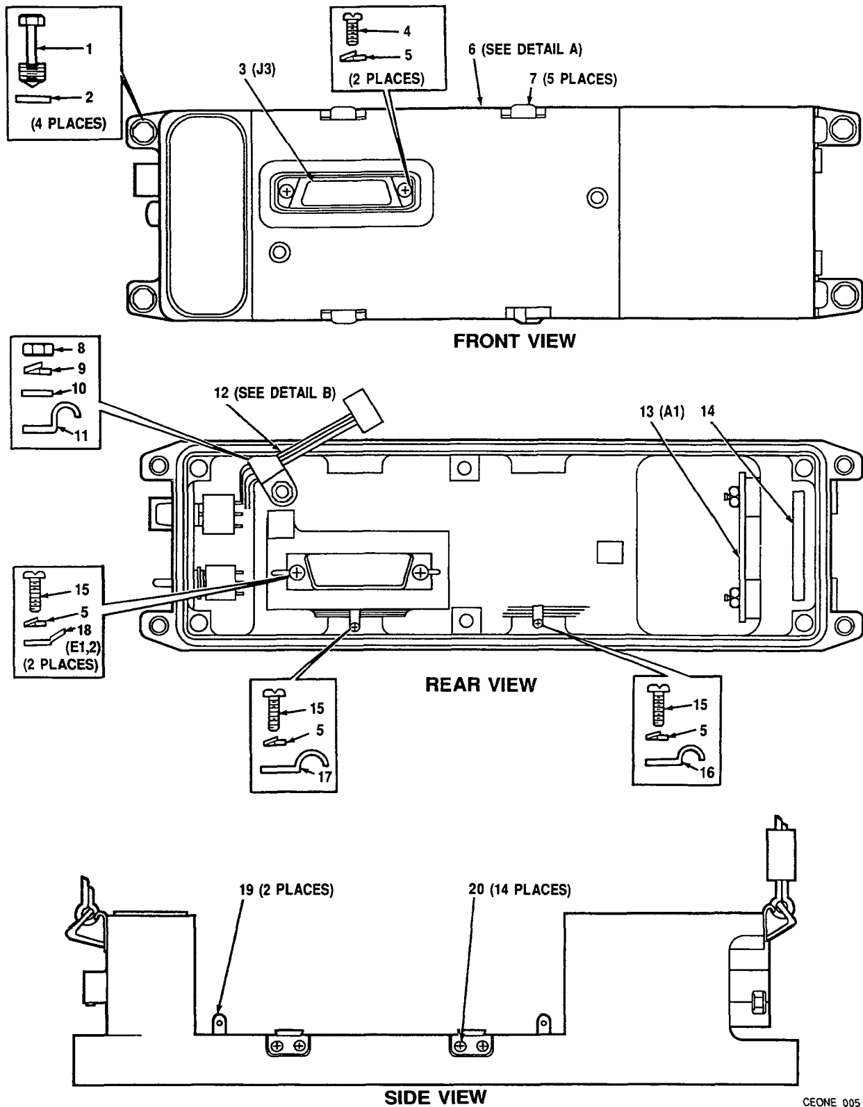
Figure 5. Front Panel Assembly A1A1A1 (A3030434) (Sheet 1 of 2)
