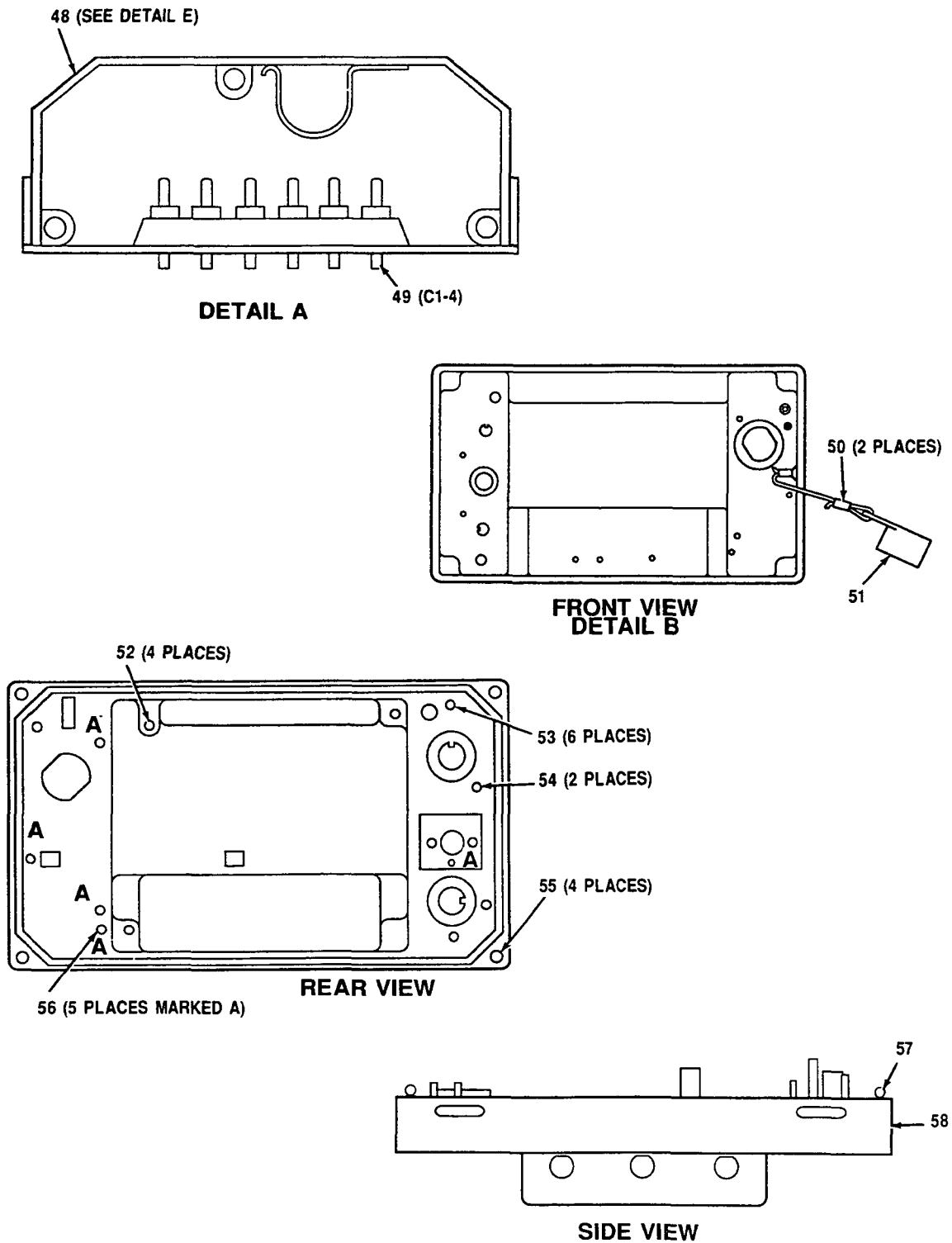
Figure 15. Front Tone converter Assembly (A3030366) (Sheet 4 of 5)
