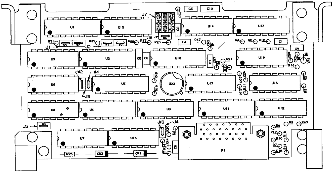
Figure 8. Timing Assembly A7 (A3024685) (Sheet 1 of 4)
