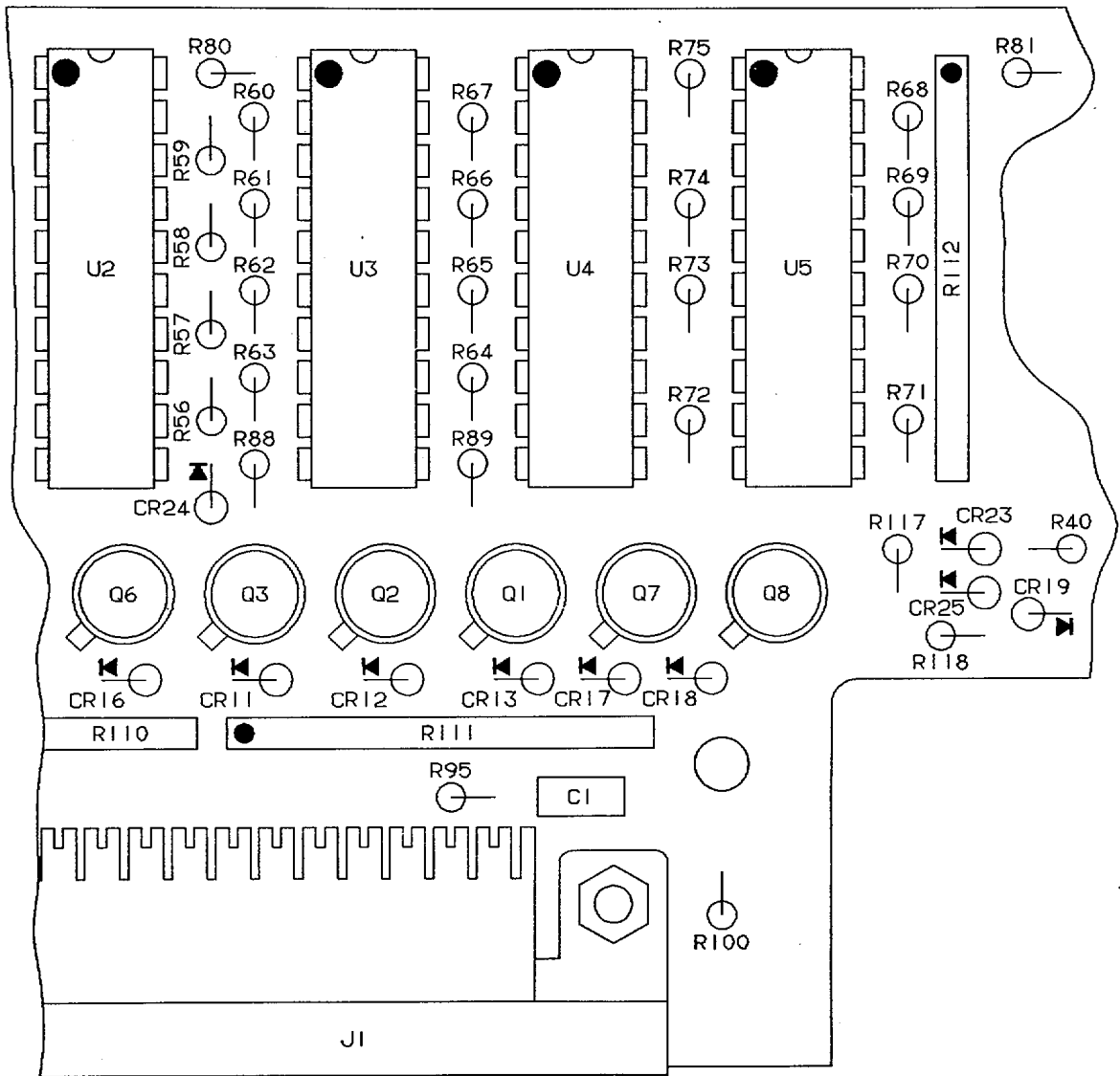
Figure 3. I/O CCA A1A1 (A3024019) (Sheet 3 of 6)
