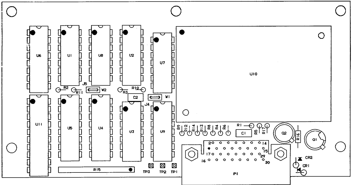
Figure 12. TSEC CCA A5A1 (A3024043) (Sheet 1 of 4)
