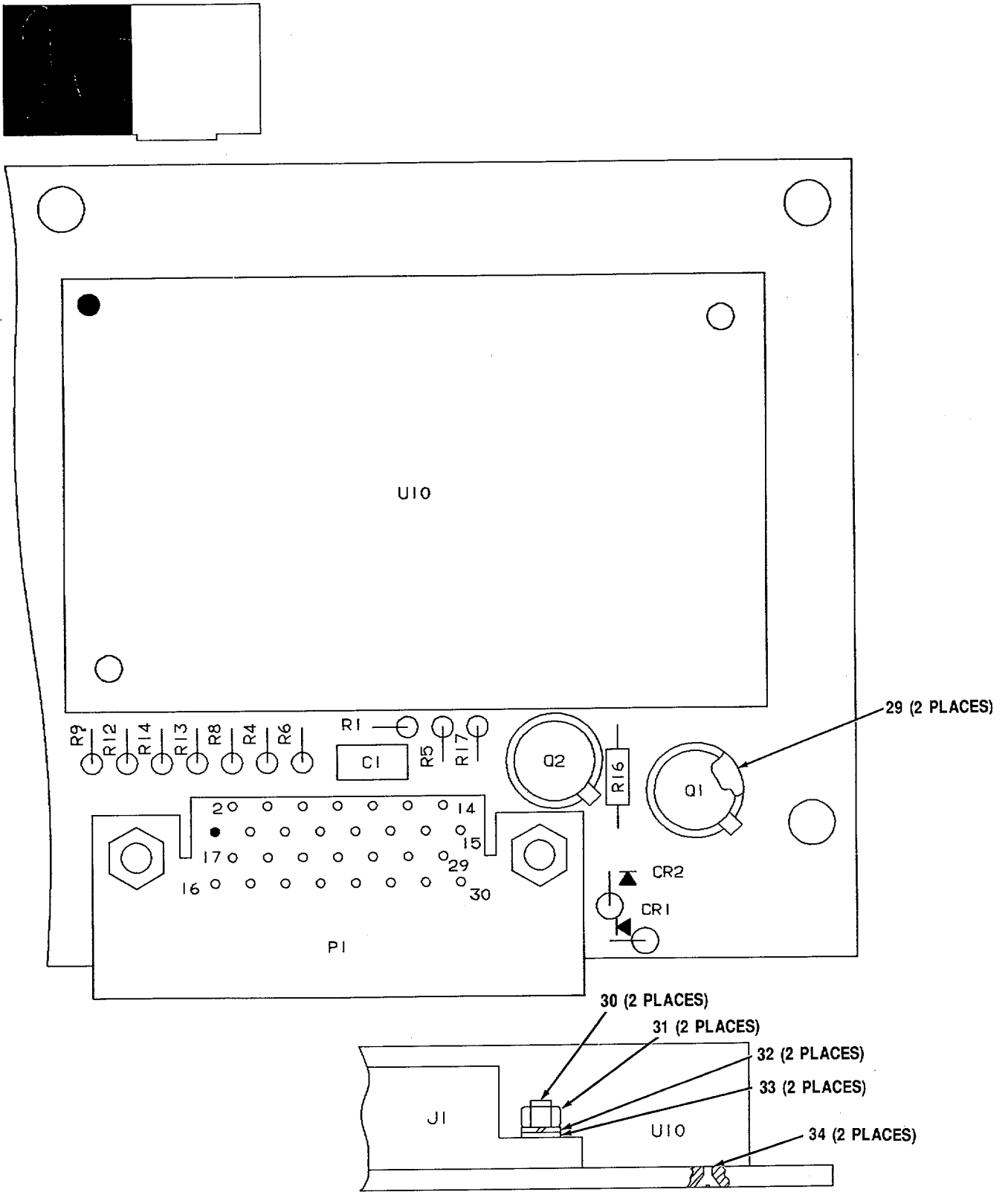
Figure 12. TSEC CCA A5A1 (A3024043) (Sheet 3 of 4)
