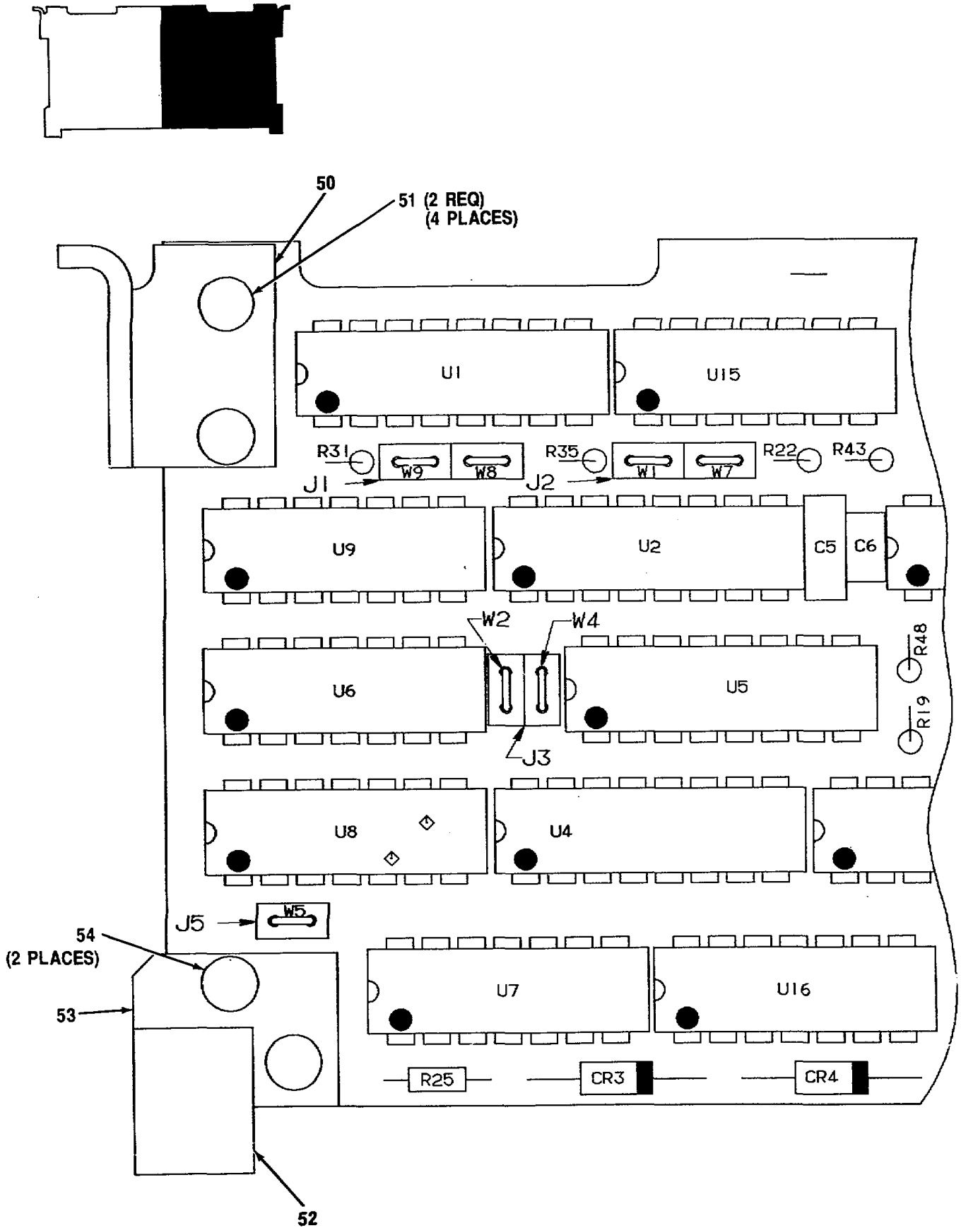
Figure 8. Timing Assembly A7 (A3024685) (Sheet 2 of 4)
