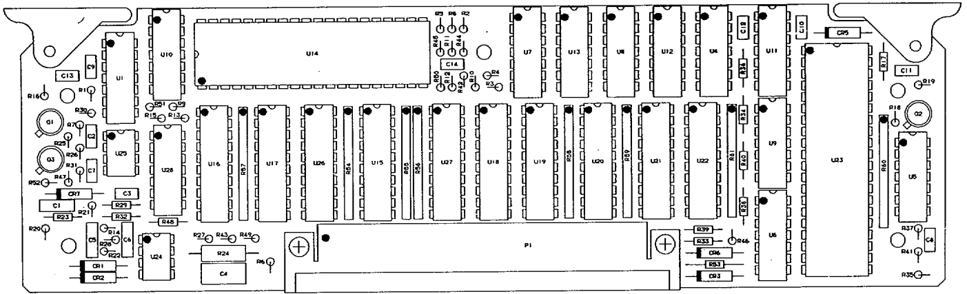
Figure 7. CPU I/O CCA A4A1 (A3024031) (Sheet 1 of 5)
