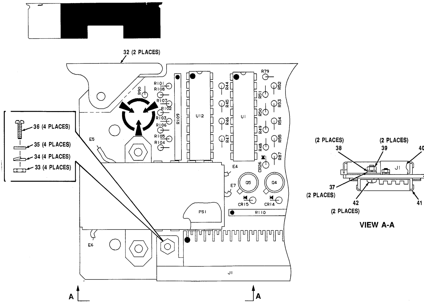
Figure 3. I/O CCA A1A1 (A3024019) (Sheet 2 of 6)
