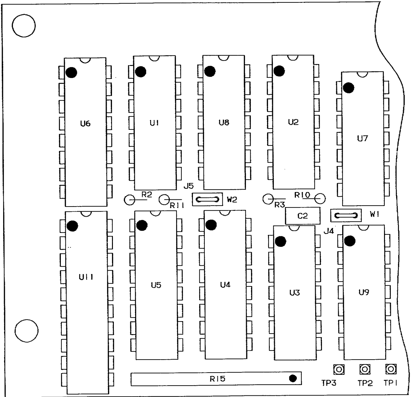
Figure 12. TSEC CCA A5A1 (A3024043) (Sheet 2 of 4)
