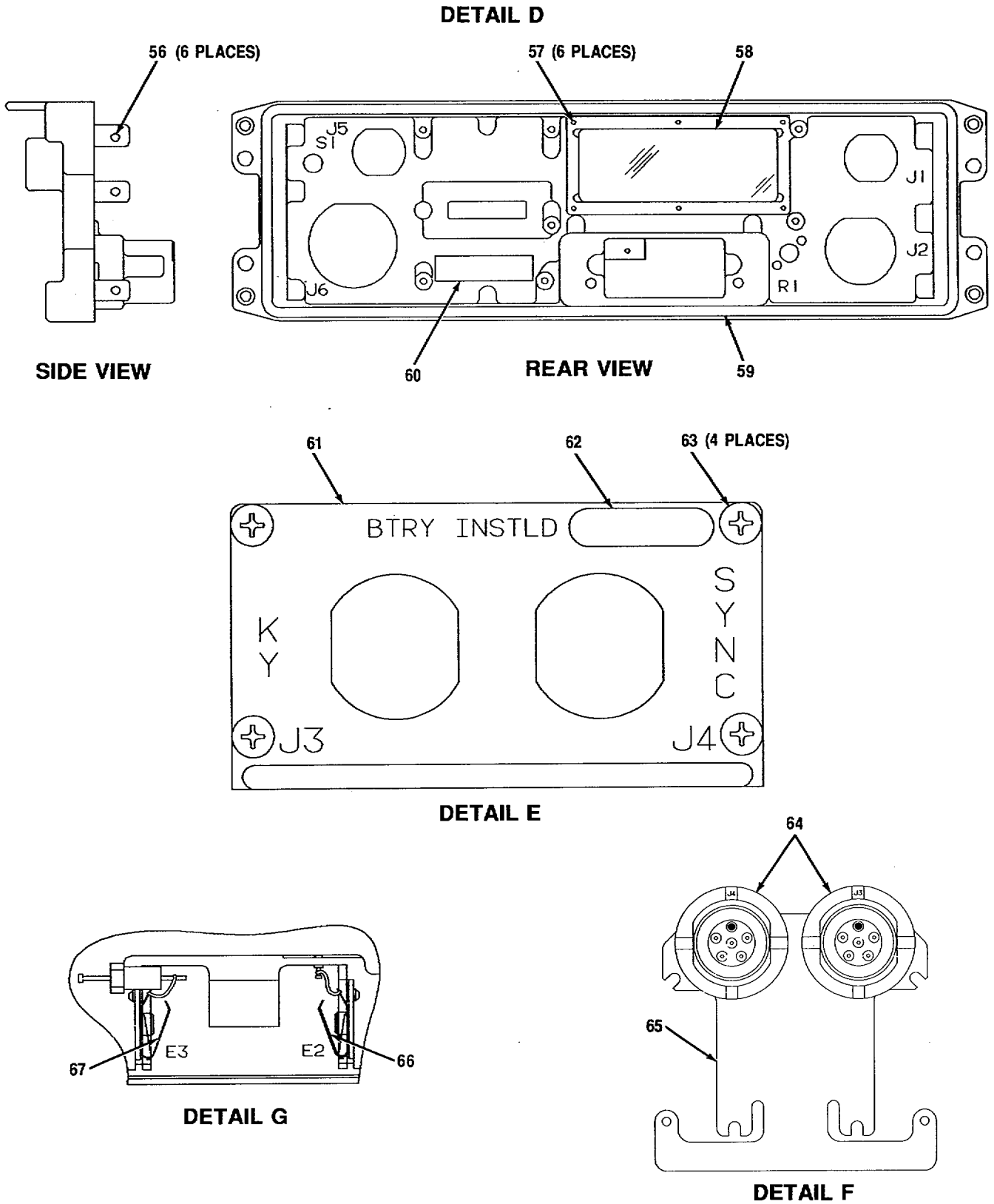
Figure 13. Panel and Chassis Assy A8 (A3024004) (Sheet 5 of 5)
