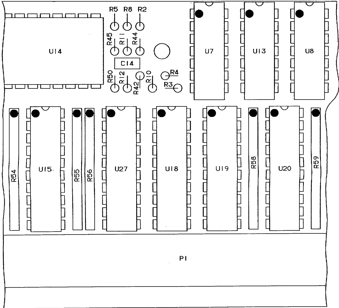
Figure 7. CPU I/O CCA A4A1 (A3024031) (Sheet 3 of 5)
