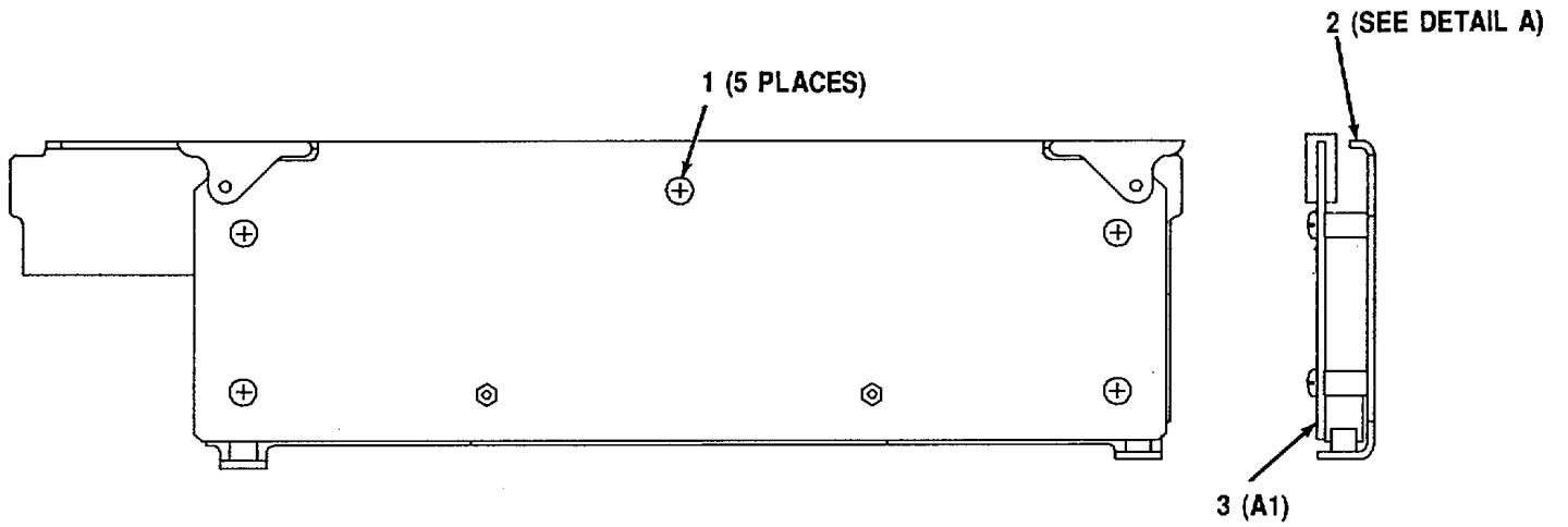
Figure 6. CPU I/O Assembly A4 (A3024029) (Sheet 1 of 2)
