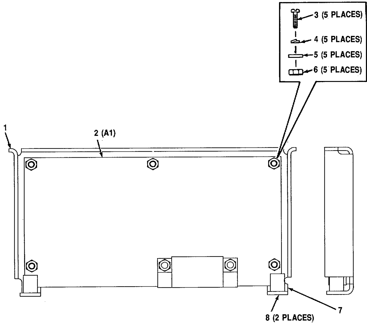
Figure 11. TSEC Assembly A5 (A3024041)
