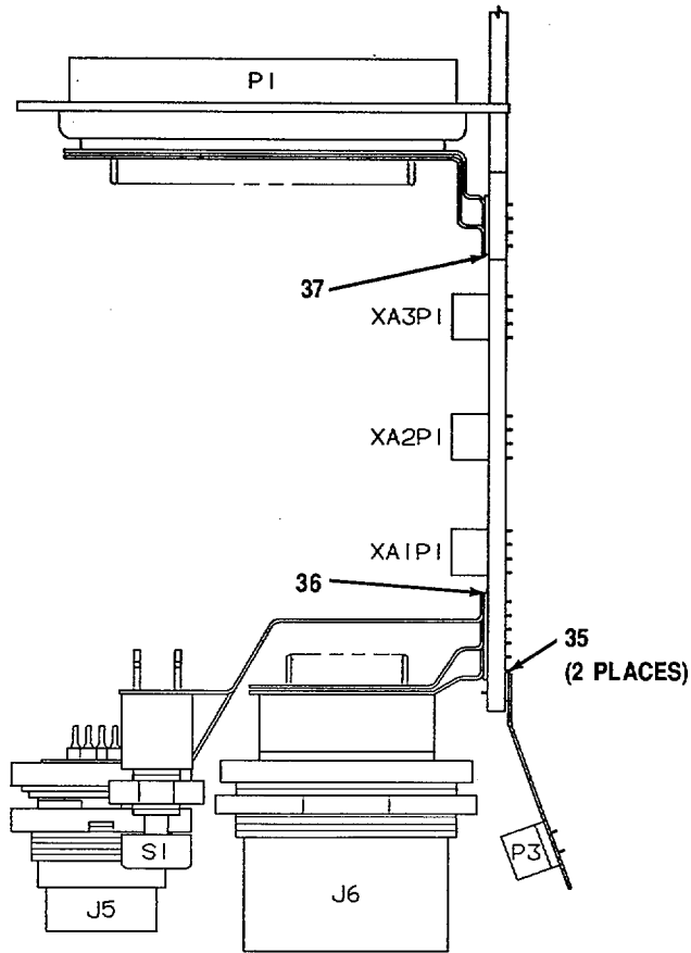
VIEW B-B
