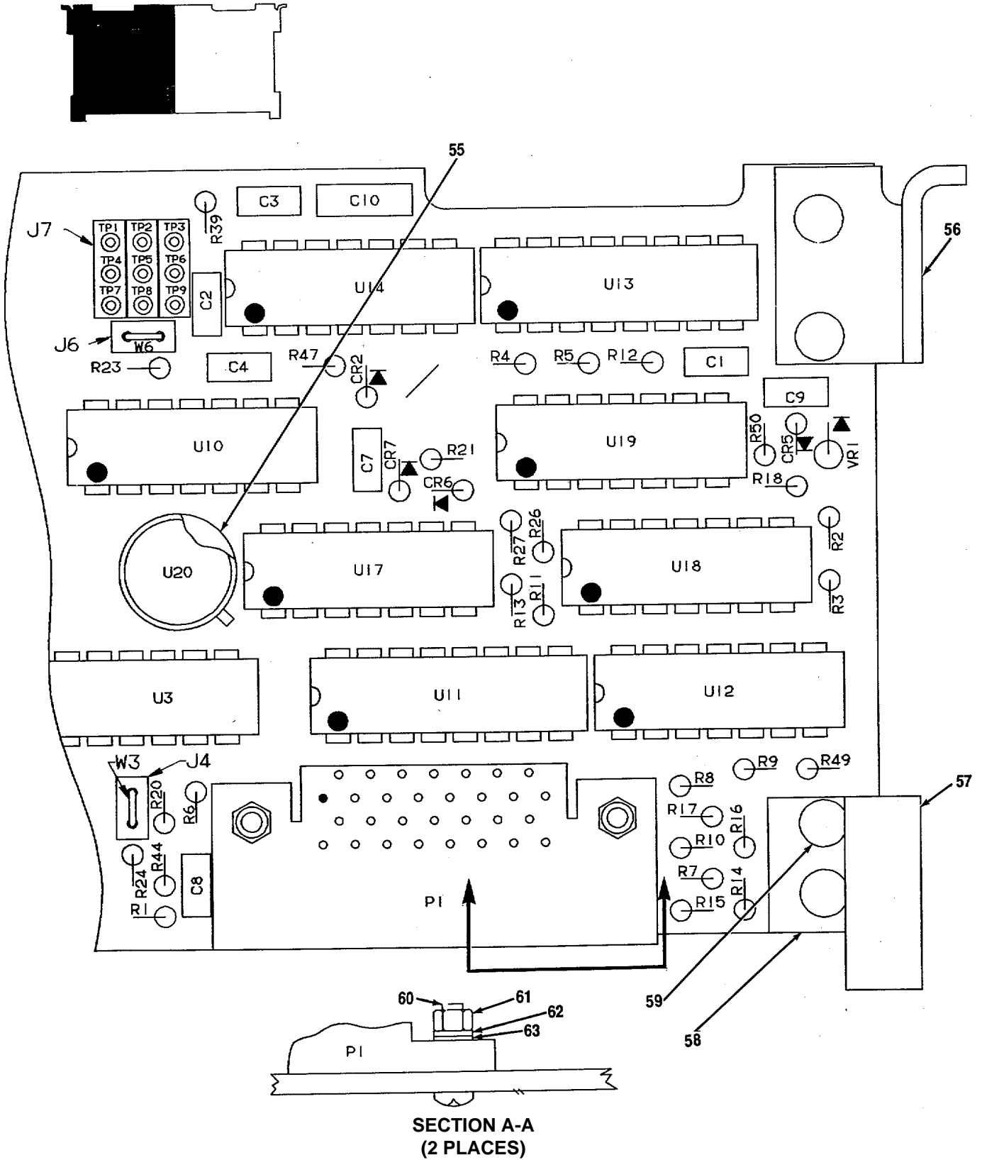
Figure 8. Timing Assembly A7 (A3024685) (Sheet 3 of 4)
