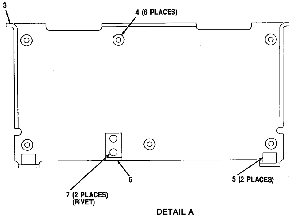
Figure 9. Power Regulator Assy A6 (A3024035)
