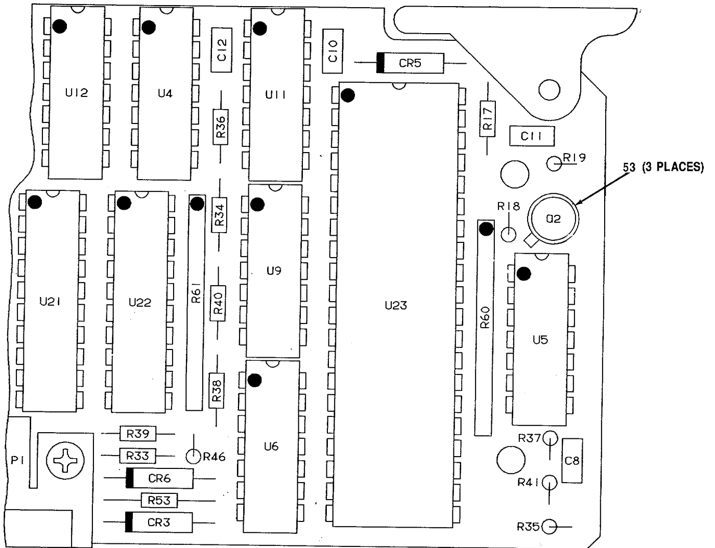
Figure 7. CPU I/O CCA A4A1 (A3024031) (Sheet 4 of 5)
