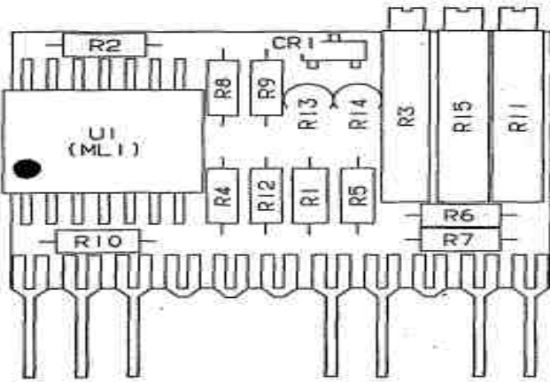
DETAIL G
