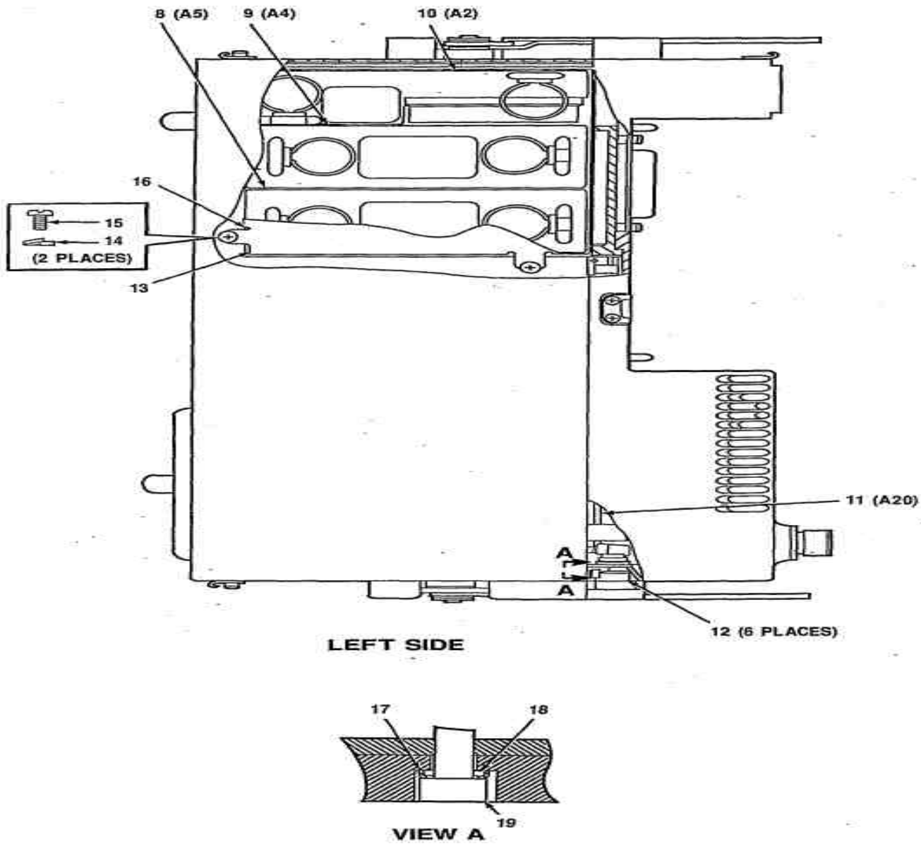
FIGURE 4 Chassis Assembly A1A2 (A3031341)
