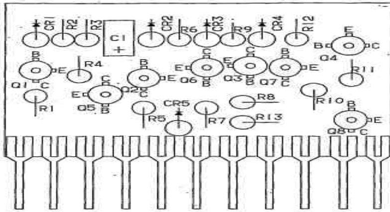
DETAIL D
