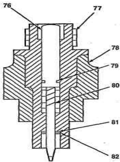
DETAIL H
