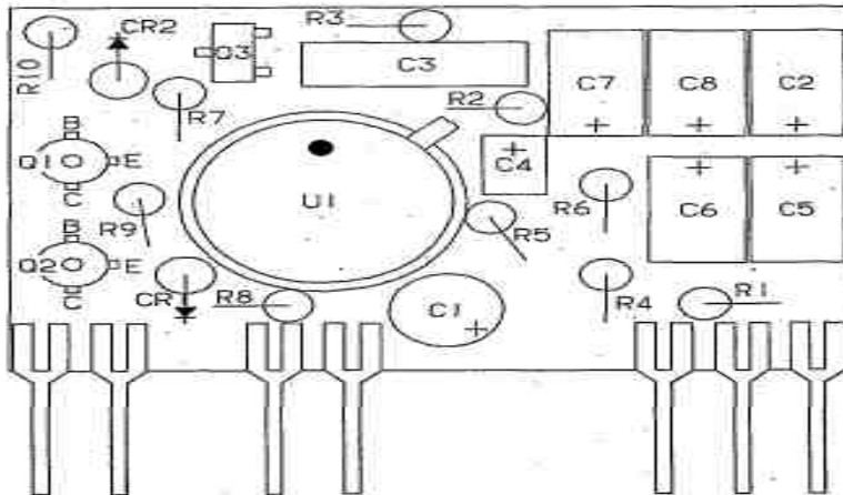
DETAIL C
