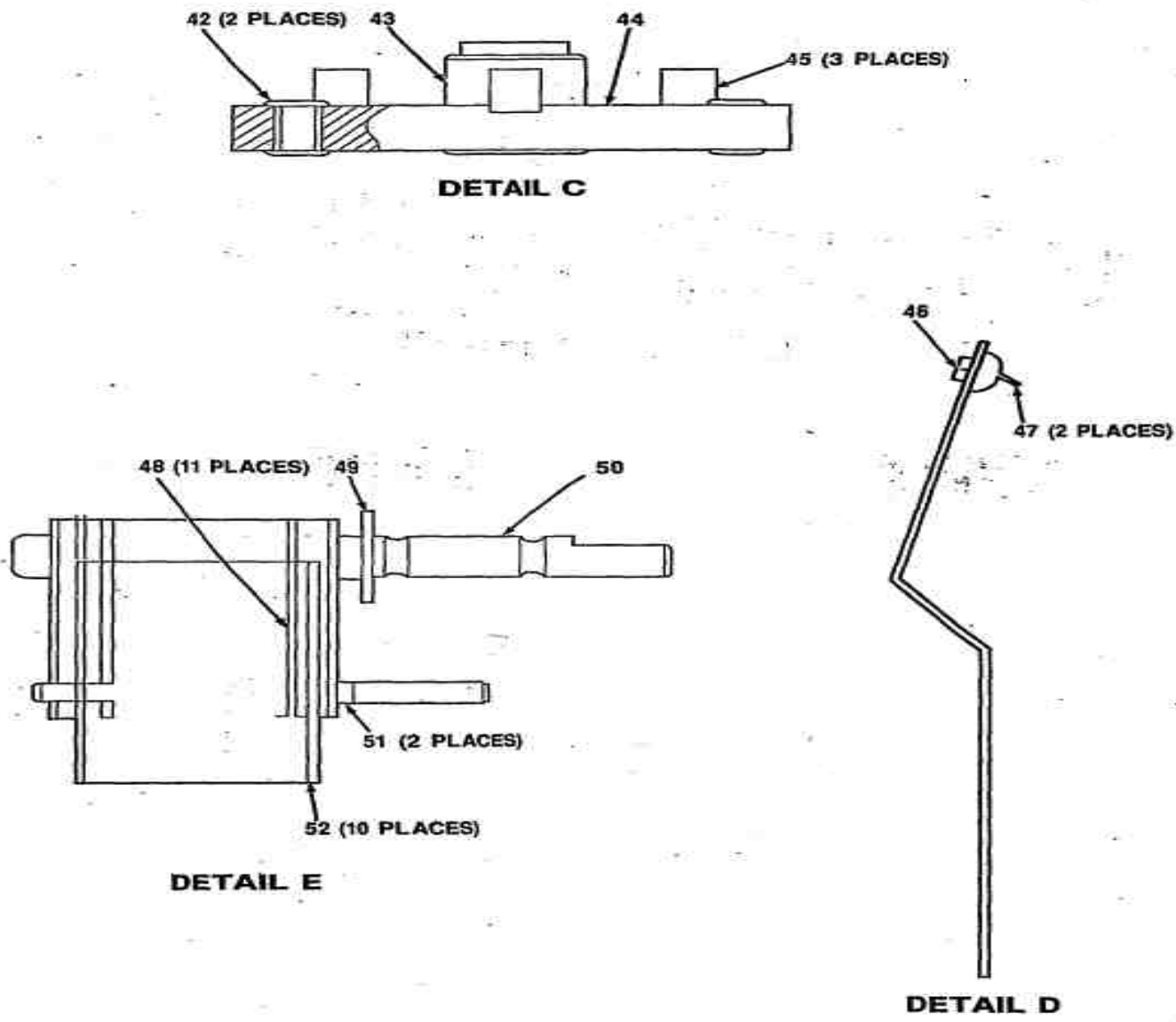
FIGURE 15 Variable Condenser Assy A1A2A20C1 (A3027653)
