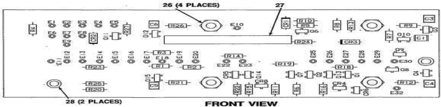
FRONT VIEW
