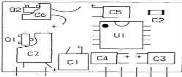
DETAIL D
