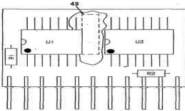
DETAIL C
