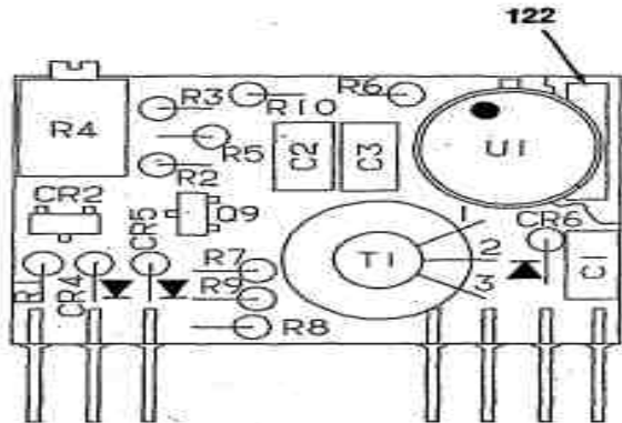
DETAIL G
