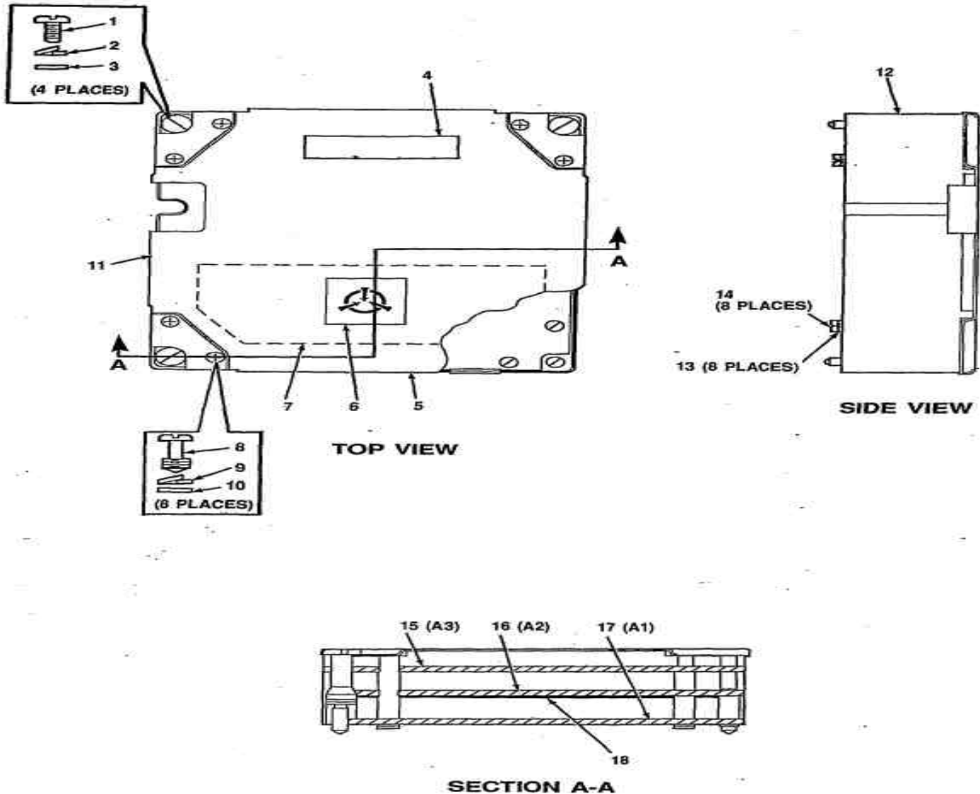
FIGURE 23 Synthesizer Module Assy A1A2A3 (A3026003)
