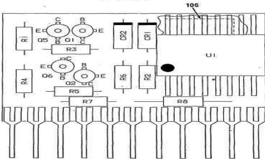
DETAIL J
