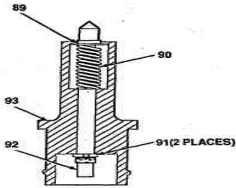
DETAIL G
