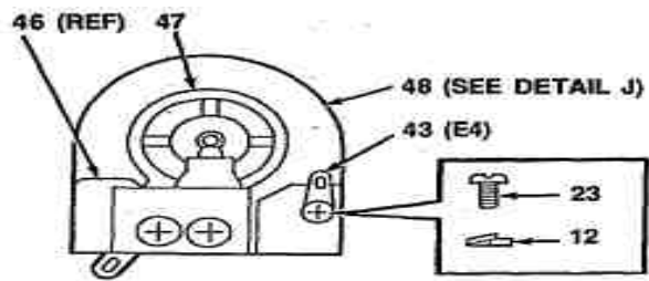
SECTION D
