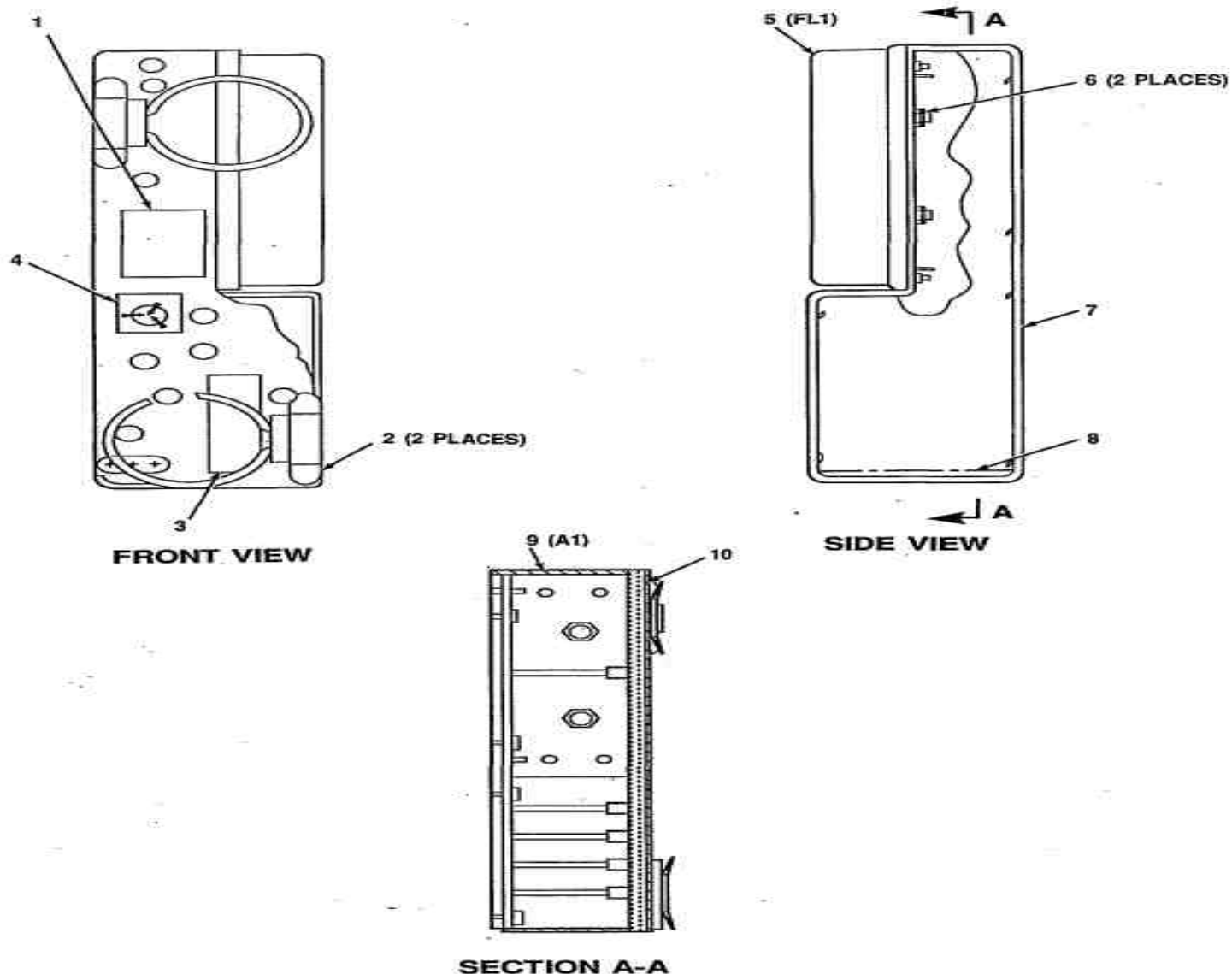
FIGURE 31 RF Translator Assy A1A2A2 (A3026004)
