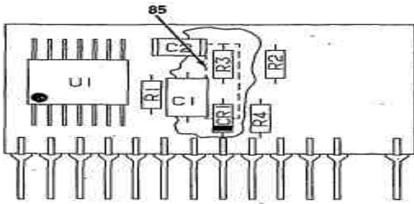
DETAIL G
