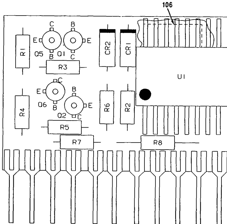
DETAIL J
