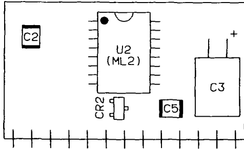
DETAIL K
