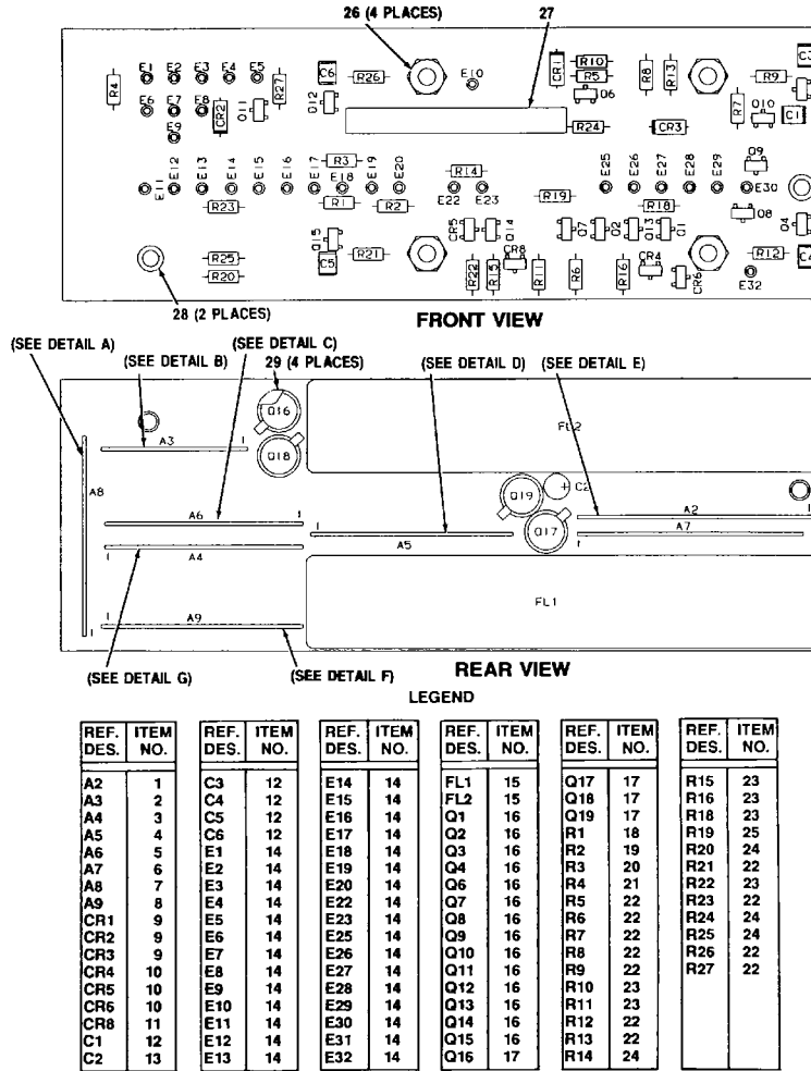
Figure 34. CCA (A3027350) (Sheet 1 of 4)
