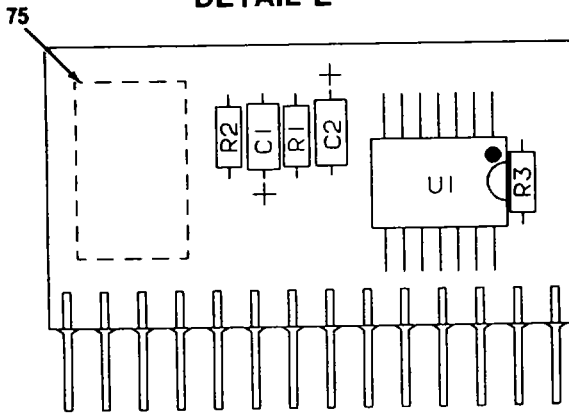
DETAIL F
