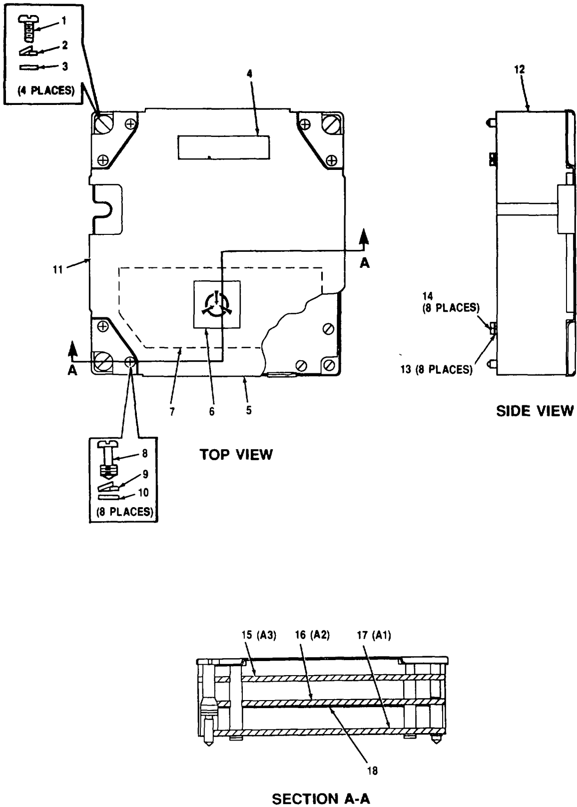
Figure 23. Synthesizer Module Assy A1A2A3 (A3026003)
