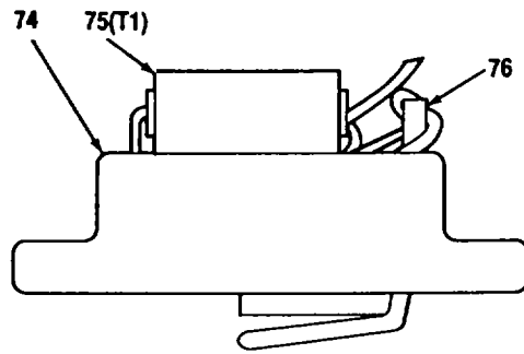
DETAIL D
