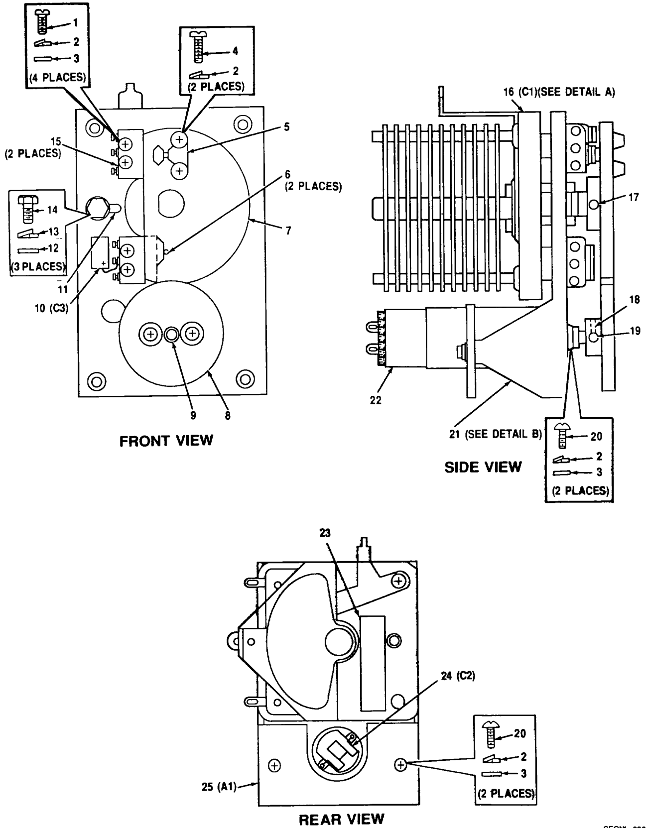
Figure 15. Variable Condenser Assy A1A2A20C1 (A3027653) (Sheet 1 of 3)
