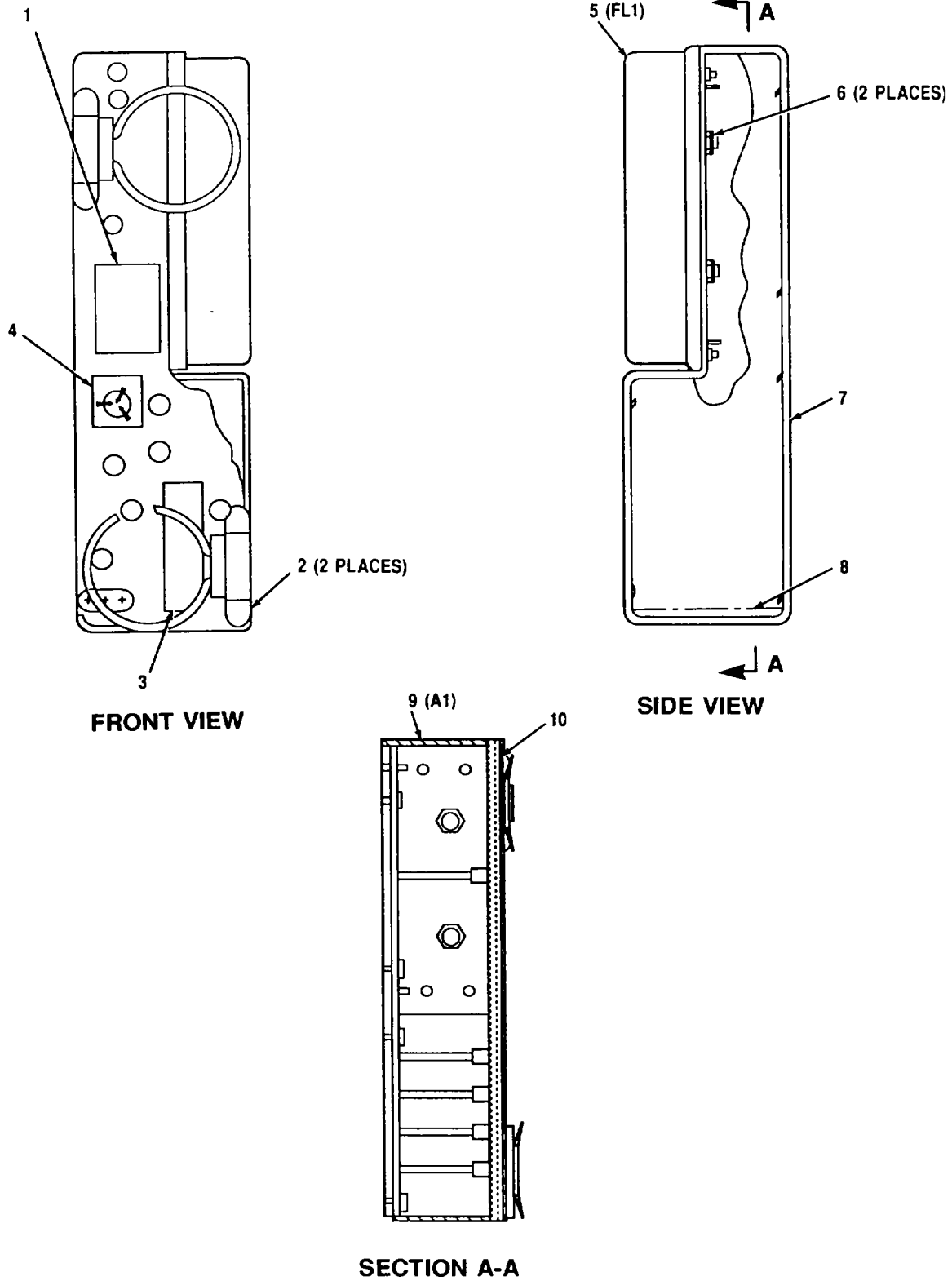
Figure 31. RF Translator Assy A1A2A2 (A3026004)
