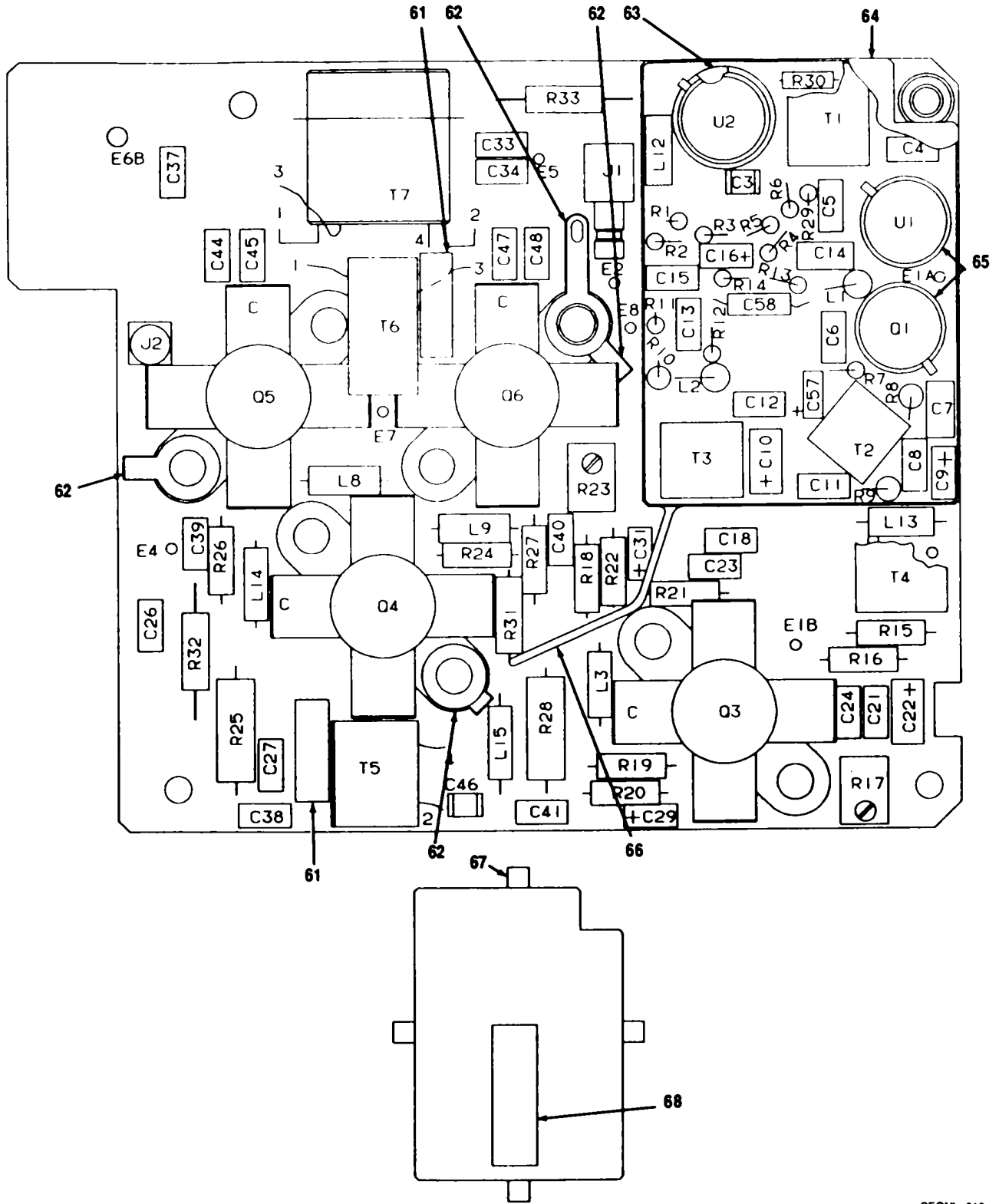
Figure 6. RF Power Amplifier CCA A1A2A1A2 (A3027322-1) (Sheet 1 of 2)
