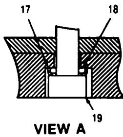
Figure 4. Chassis Assembly A1A2 (A3031341) (Sheet 2 of 2)
