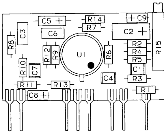
DETAIL E
