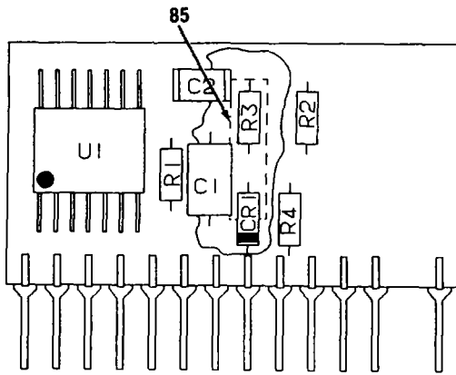
DETAIL G
