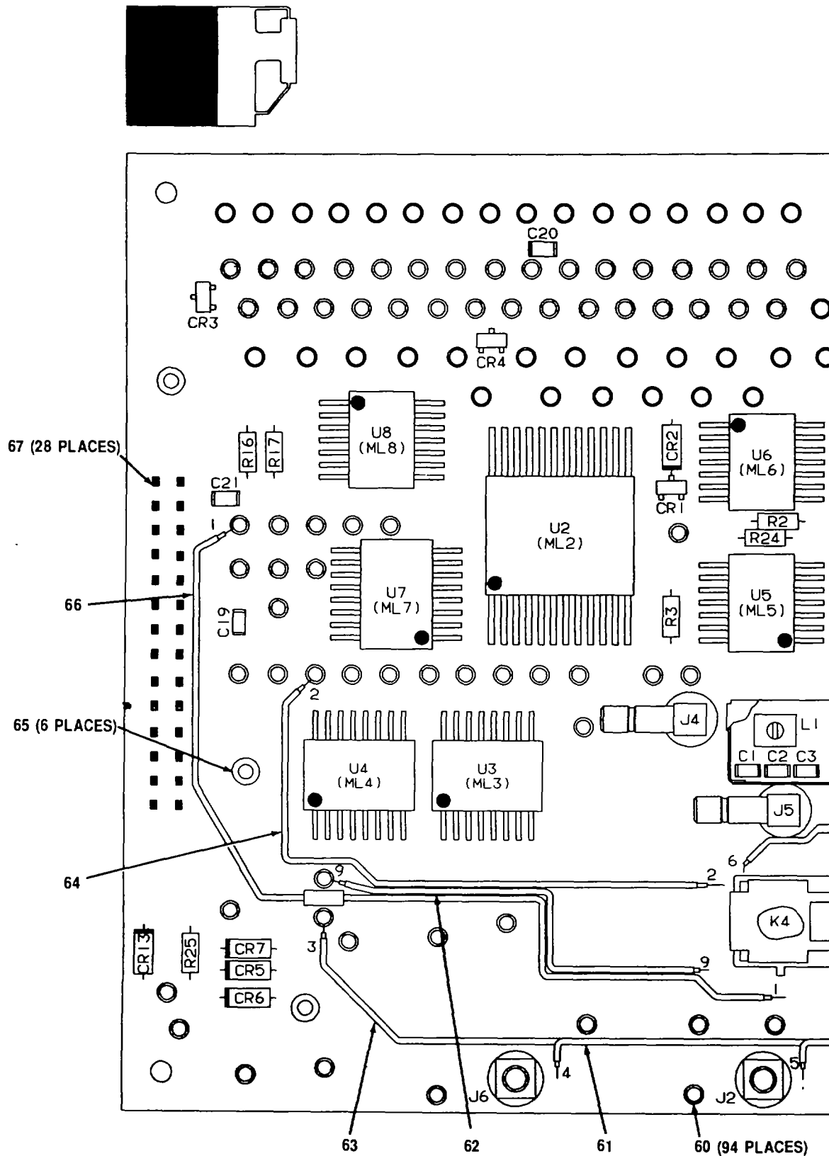
Figure 17. Grandmother Board CCA A1A2A20A12 (A3027352) (Sheet 2 of 3)
