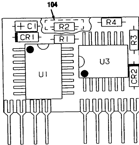
DETAIL F
