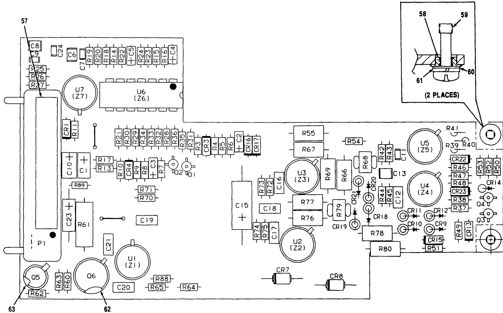
Figure 37. Servo Amp CCA A1A2A6 (A3026007) (Sheet 1 of 2)
