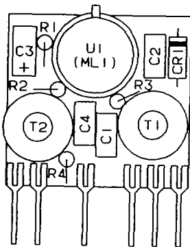
DETAIL B
