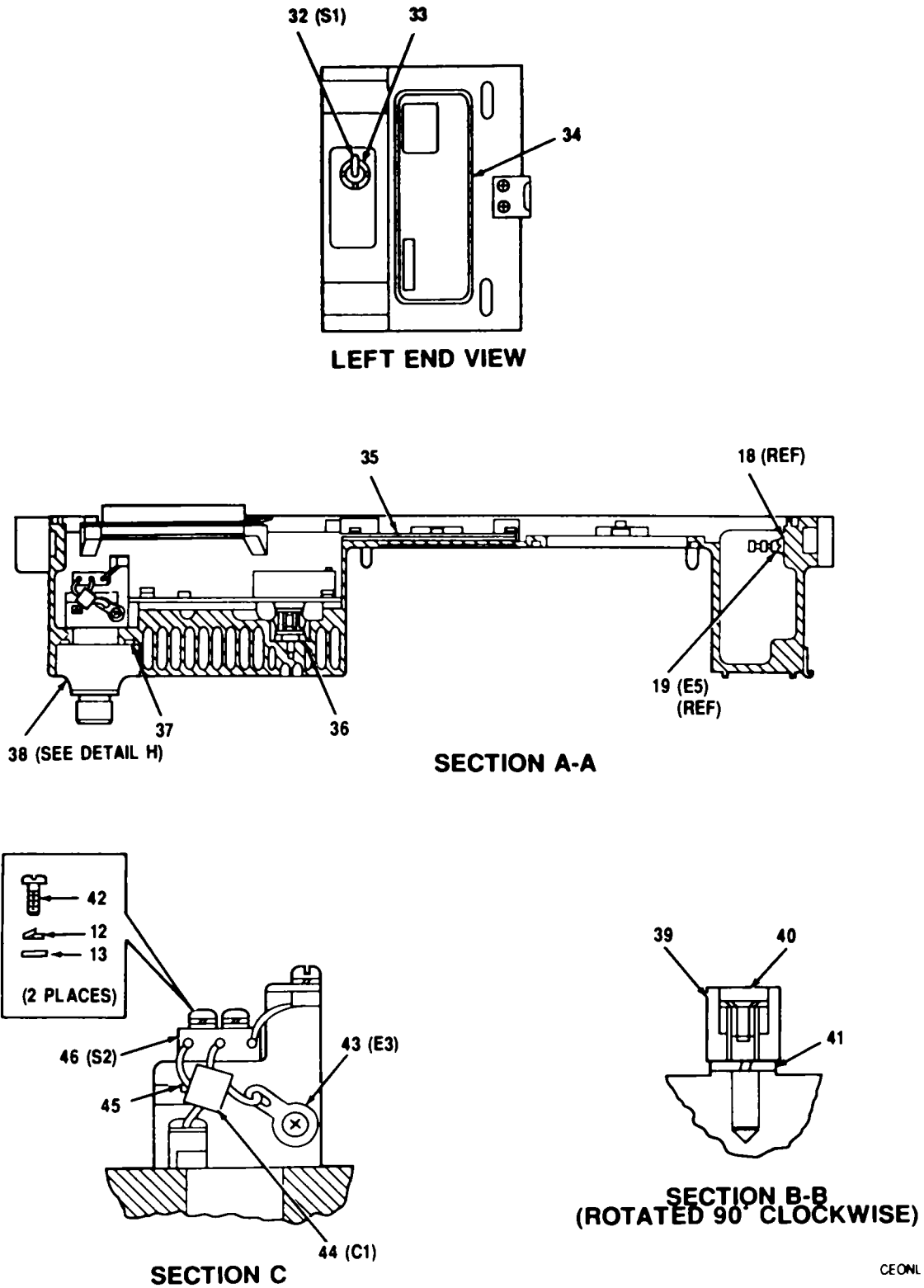
Figure 5. Front Panel Assembly A1A2A1 (A3026002) (Sheet 2 of 5)
