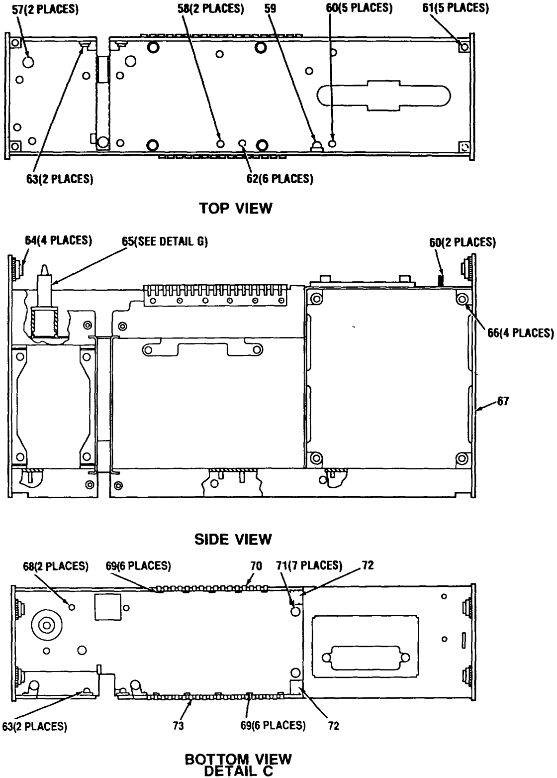
Figure 8. Receiver Exciter Chassis A1A2A20 (A3026000) (Sheet 4 of 6)
