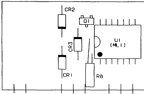
DETAIL F
