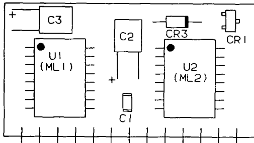
DETAIL H
