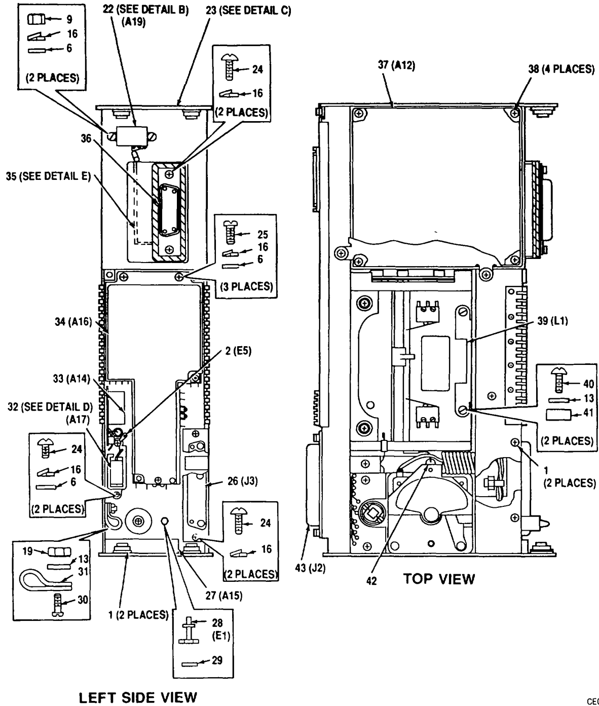
Figure 8. Receiver Exciter Chassis A1A2A20 (A3026000) (Sheet 2 of 6)
