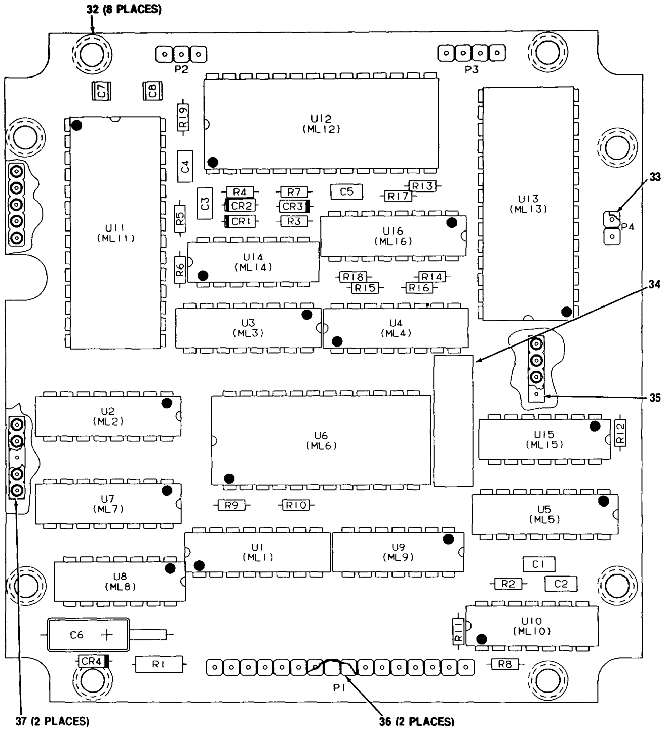
Figure 29. Data Receiver and Logic CCA (A3027687) (Sheet 1 of 2)
