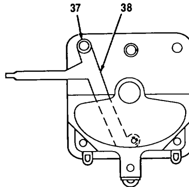
FRONT VIEW DETAIL A
