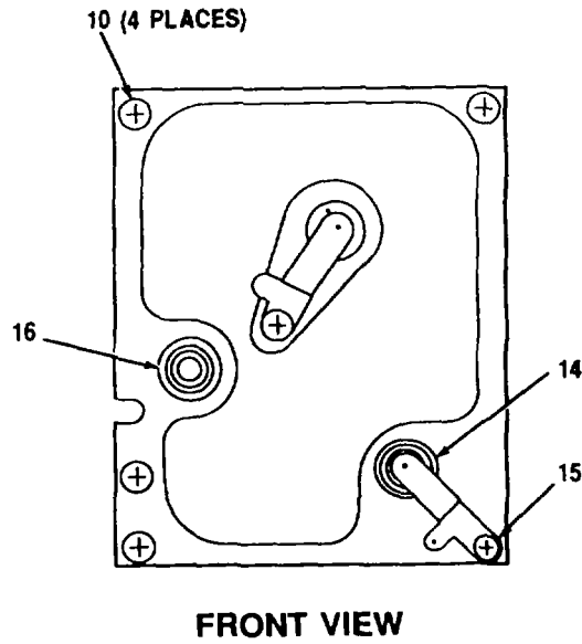
Figure 21. Coil Assy (A3030152) (Sheet 1 of 3)
