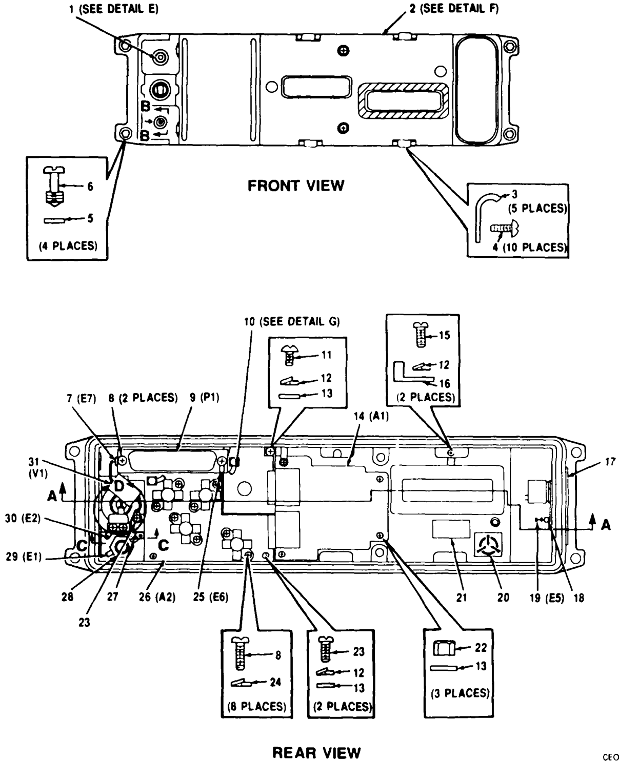
Figure 5. Front Panel Assembly A1A2A1 (A3026002) (Sheet 1 of 5)
