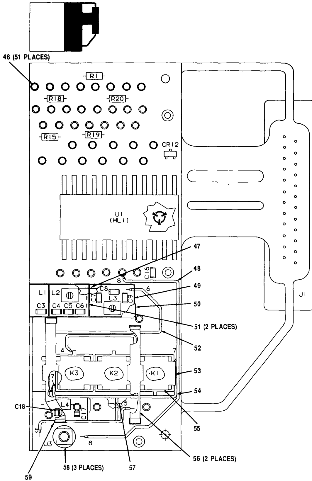
Figure 17. Grandmother Board CCA A1A2A20A12 (A3027352) (Sheet 1 of 3)
