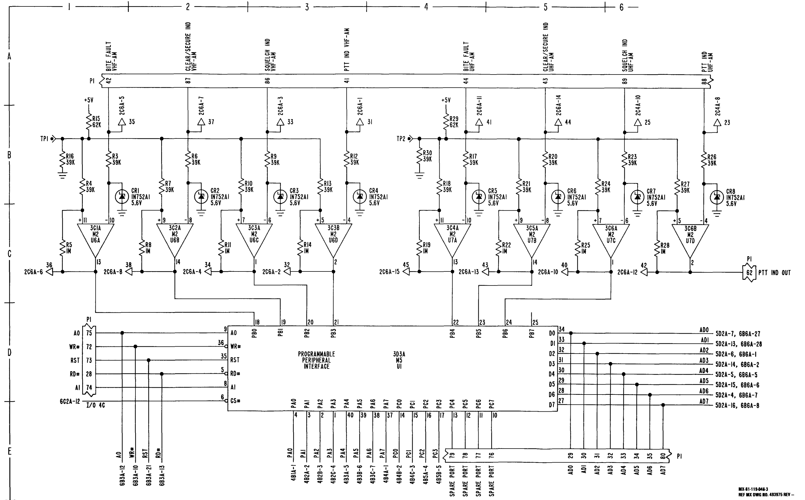
FO-4. SDU Red Interface Schematic Diagram (Sheet 3 of 6)
