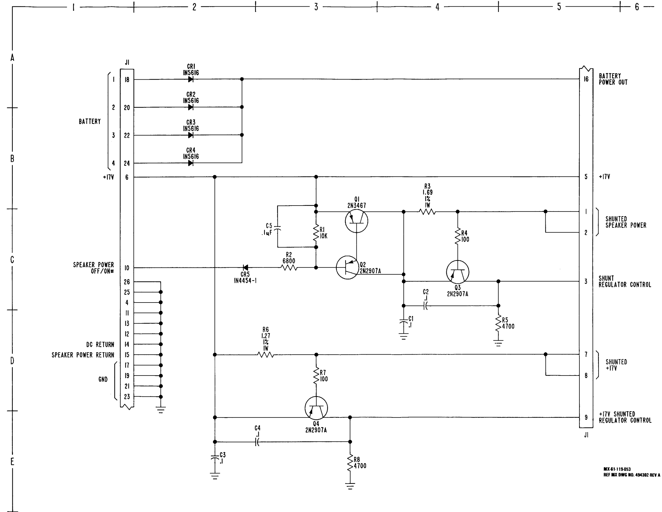
FO-11. RSC Regulator Schematic Diagram
