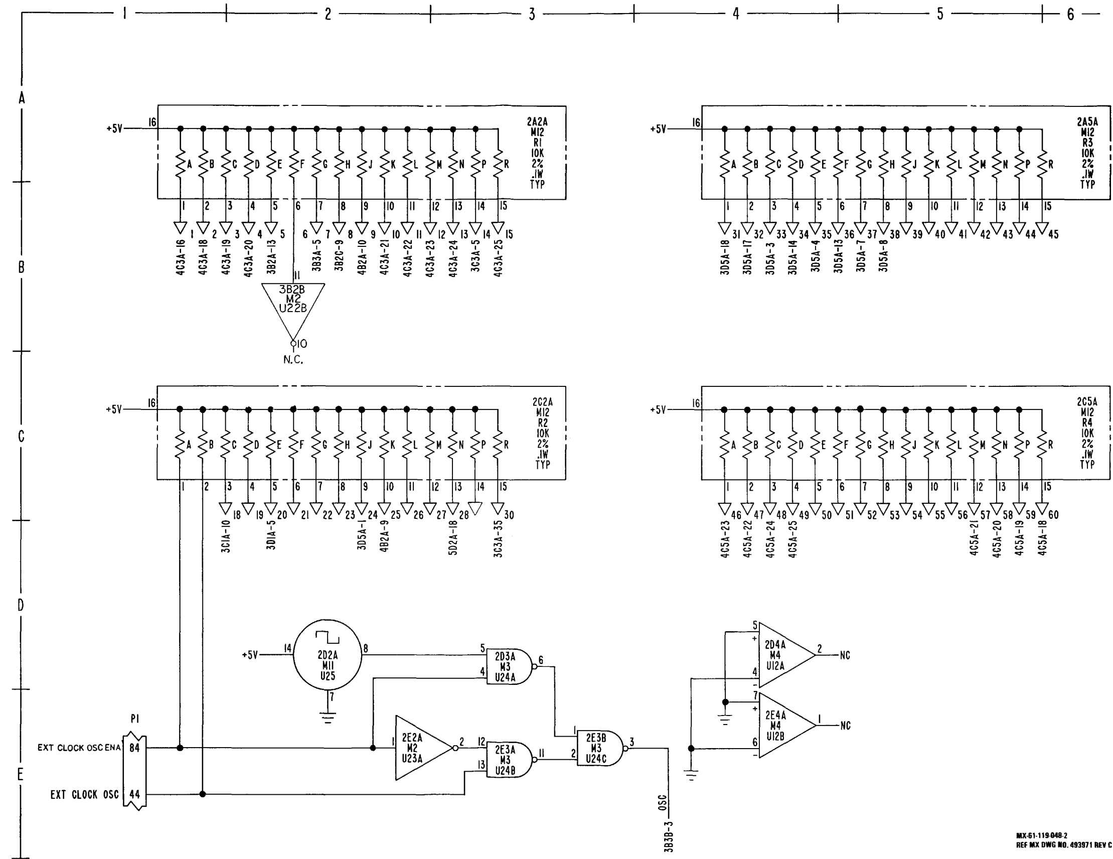
FO-6. CPU Schematic Diagram (Sheet 2 of 6)
