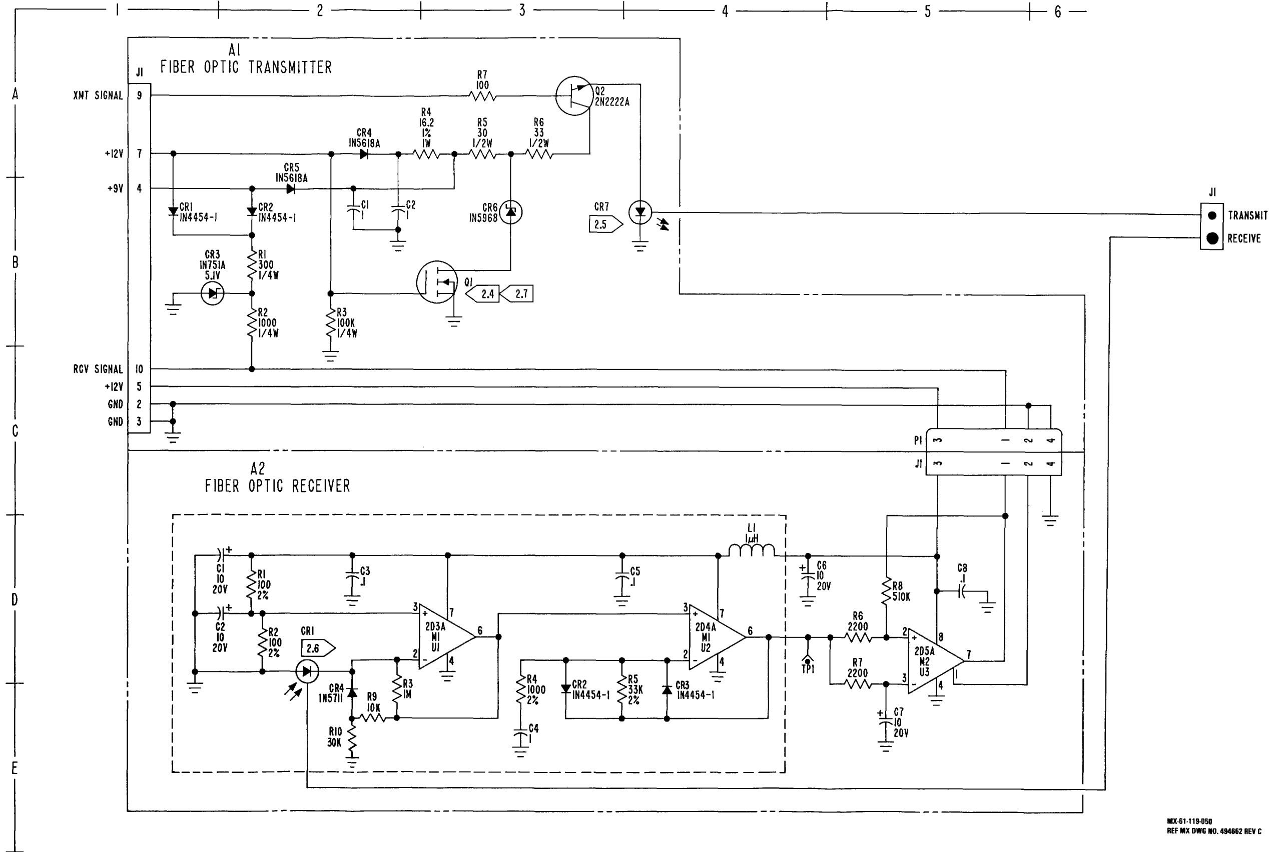
FO-8. Fiber Optic Module Assembly Schematic Diagram
