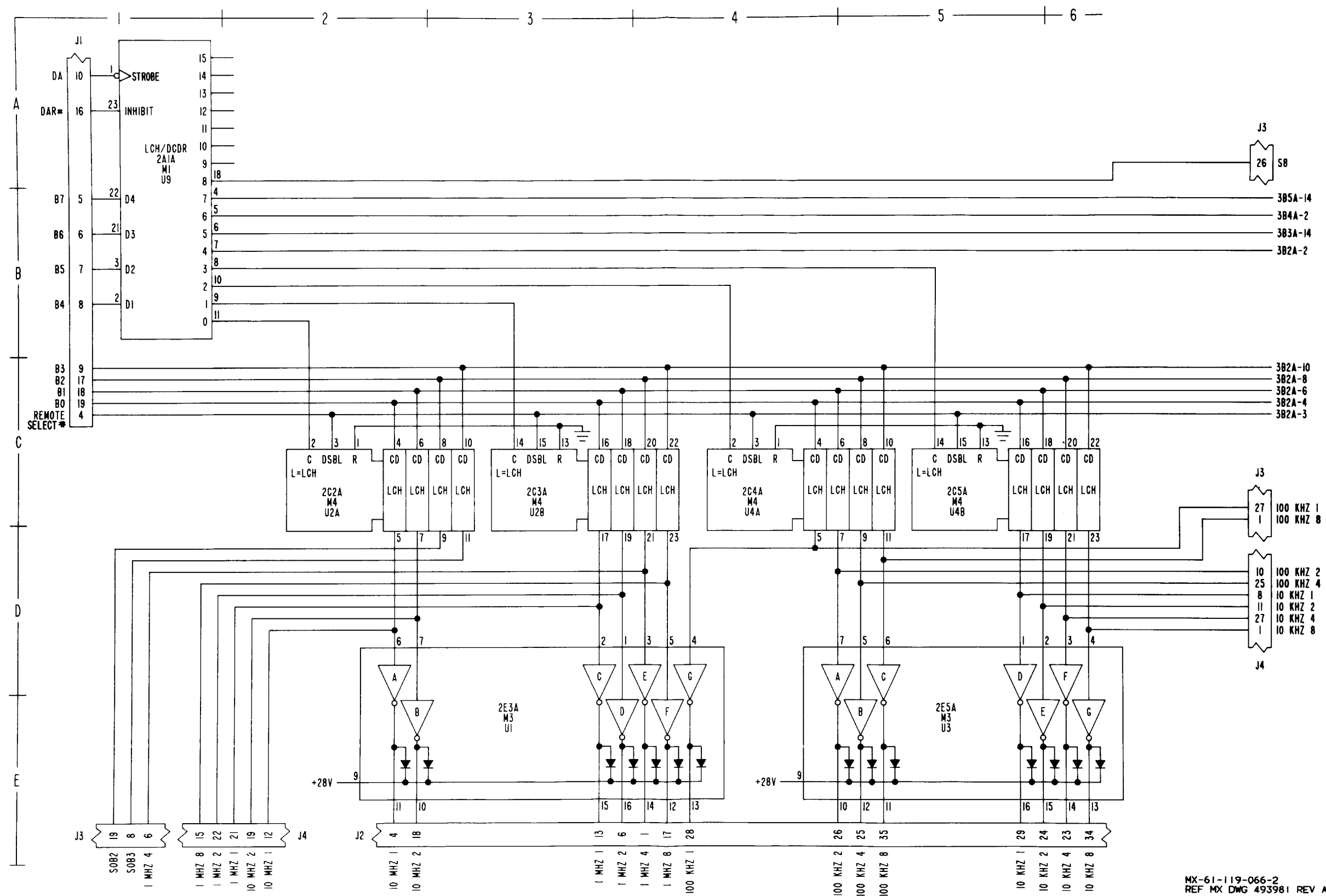
FO-20. RT Interface Schematic Diagram (Sheet 2 of 3)
