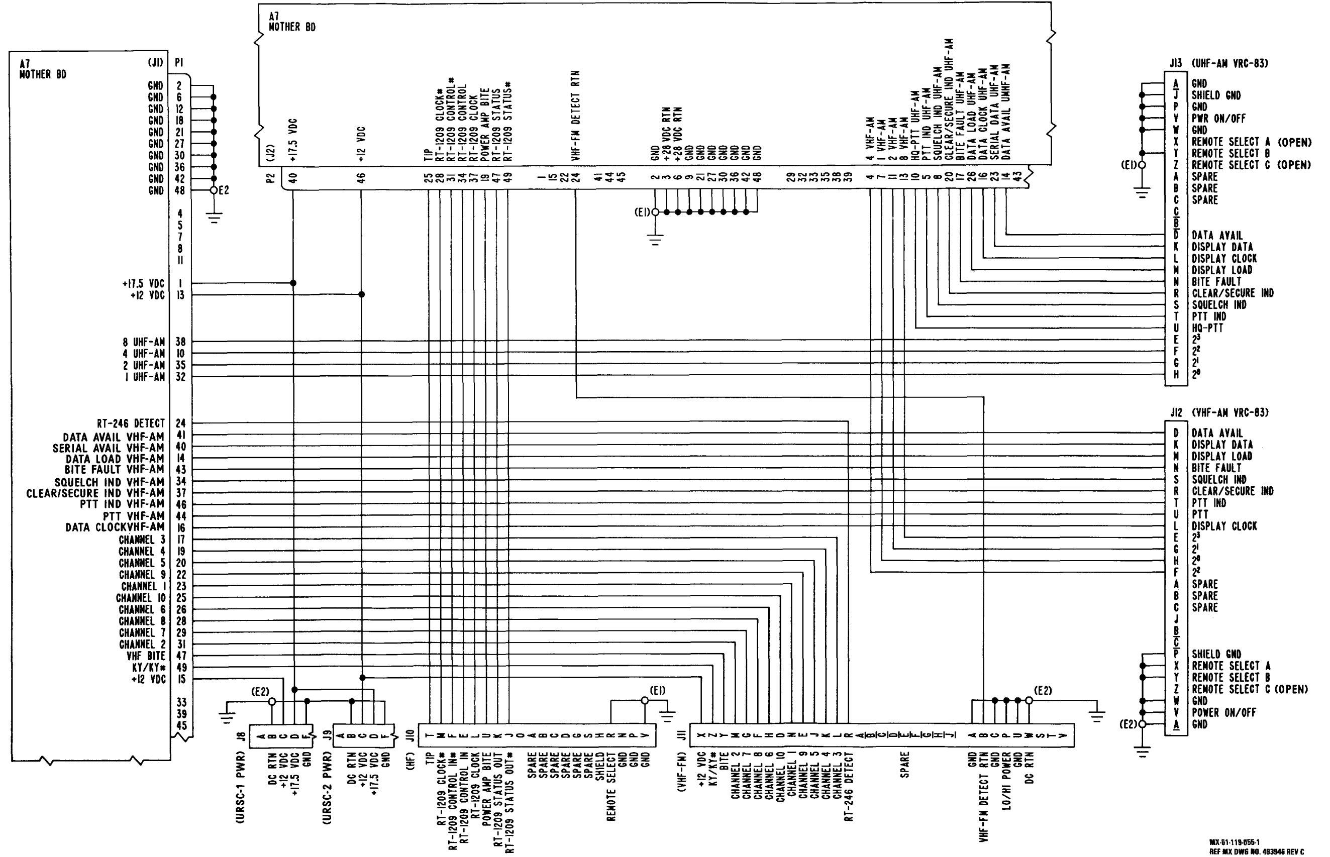
FO-13. Signal Distribution Unit Schematic Diagram (Sheet 1 of 2)
