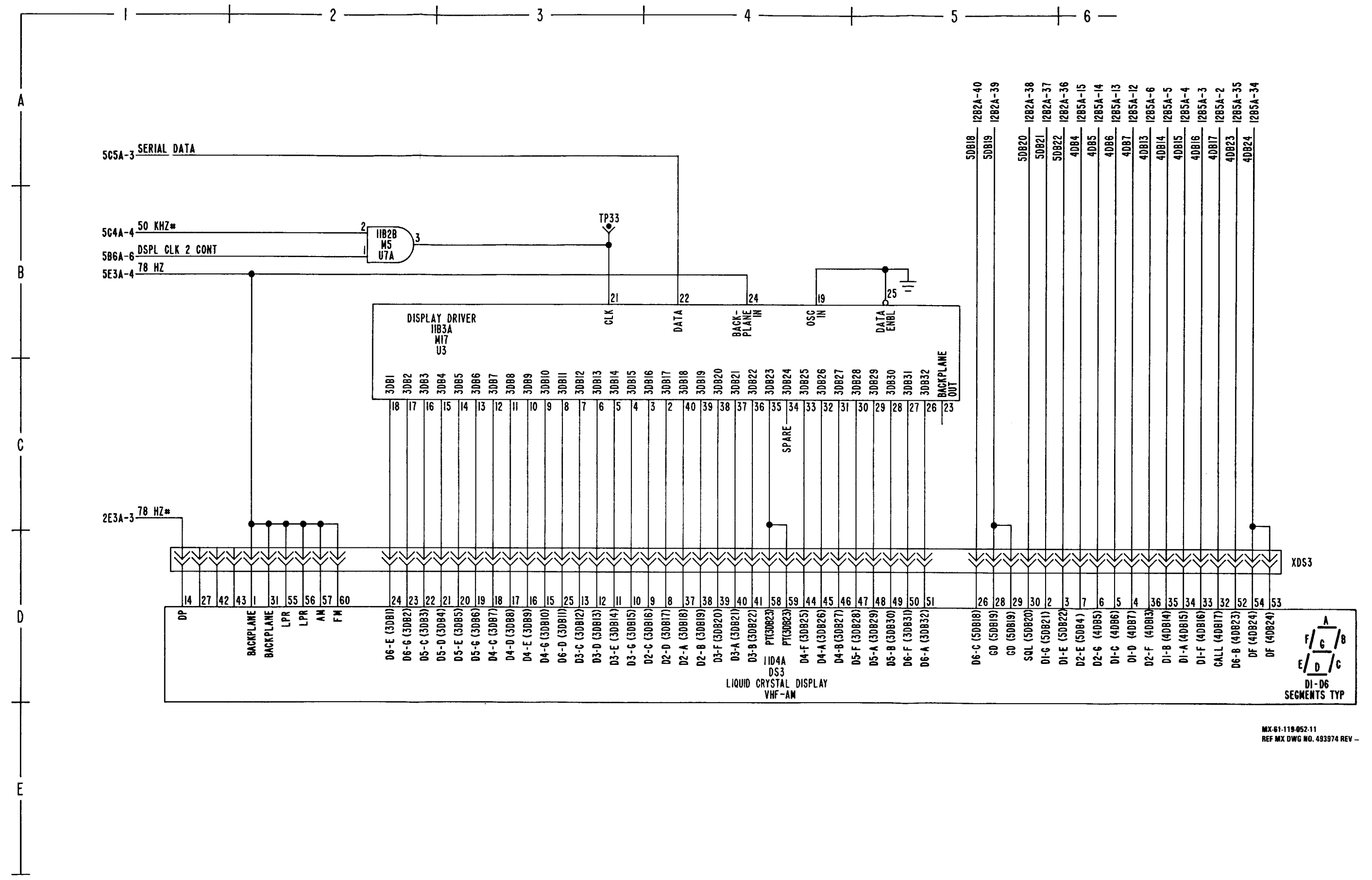
FO-10. RSC Digital Interface Schematic Diagram (Sheet 11 of 12)
