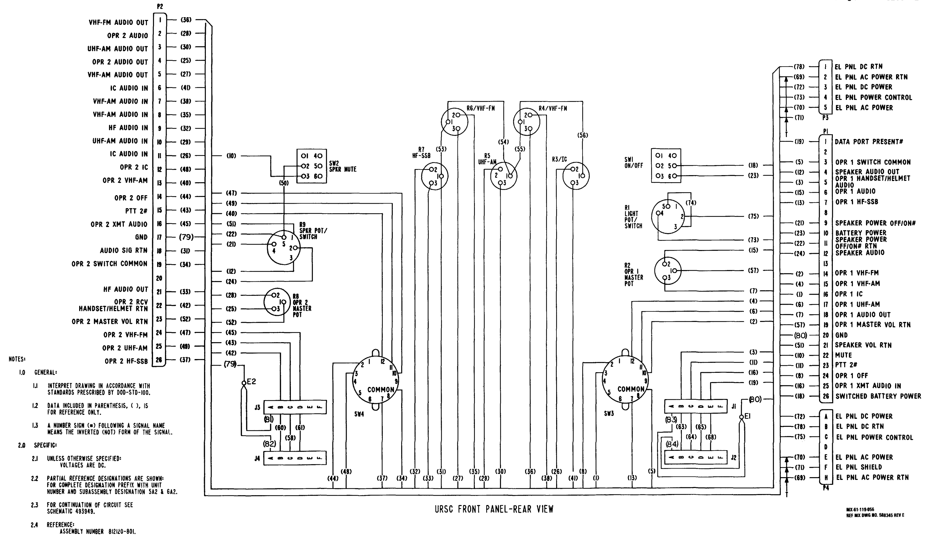
FO-14. RSC Front Panel Wiring Diagram
