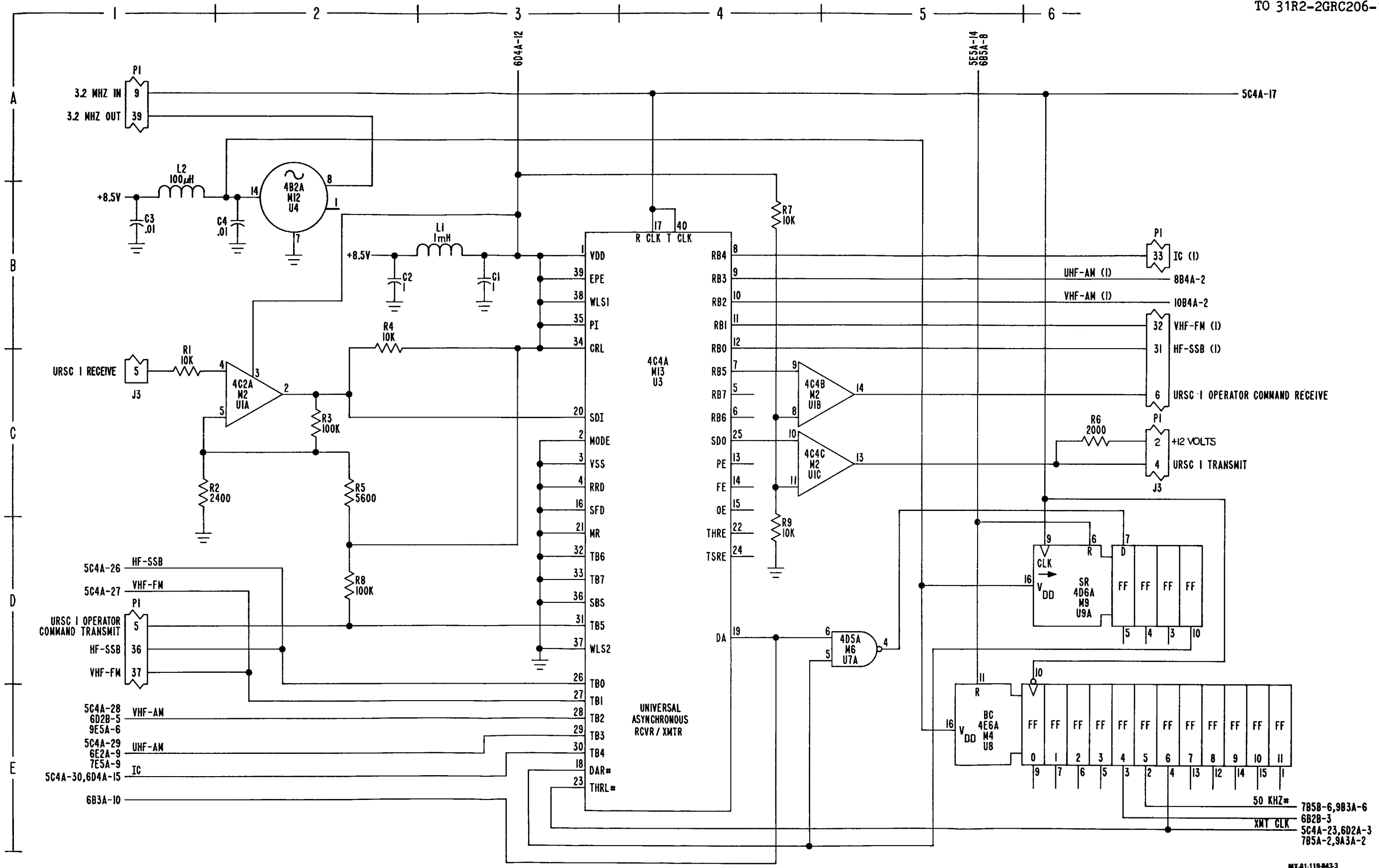
FO-2. SDU Audio Interface (1) Schematic Diagram (Sheet 3 of 9)
