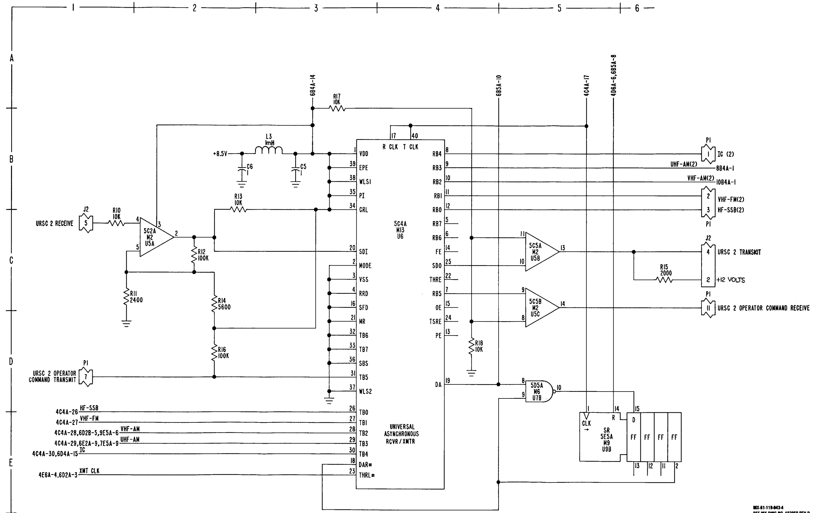
FO-2. SDU Audio Interface (1) Schematic Diagram (Sheet 4 of 9)
