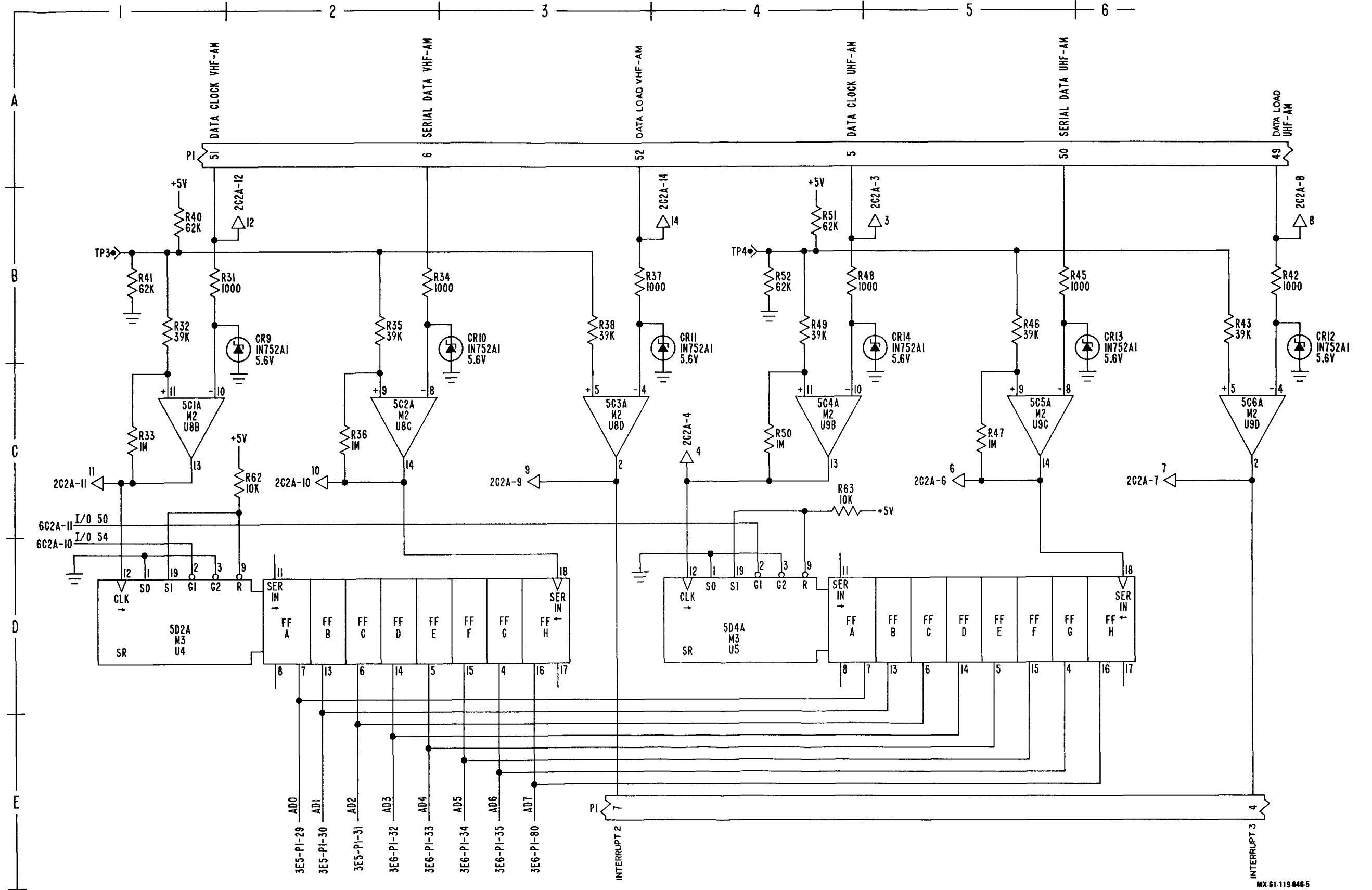
MX 61-119-046-5 REF MX DWG NO. 493975 REV D FO-4. SDU Red Interface Schematic Diagram (Sheet 5 of 6)
