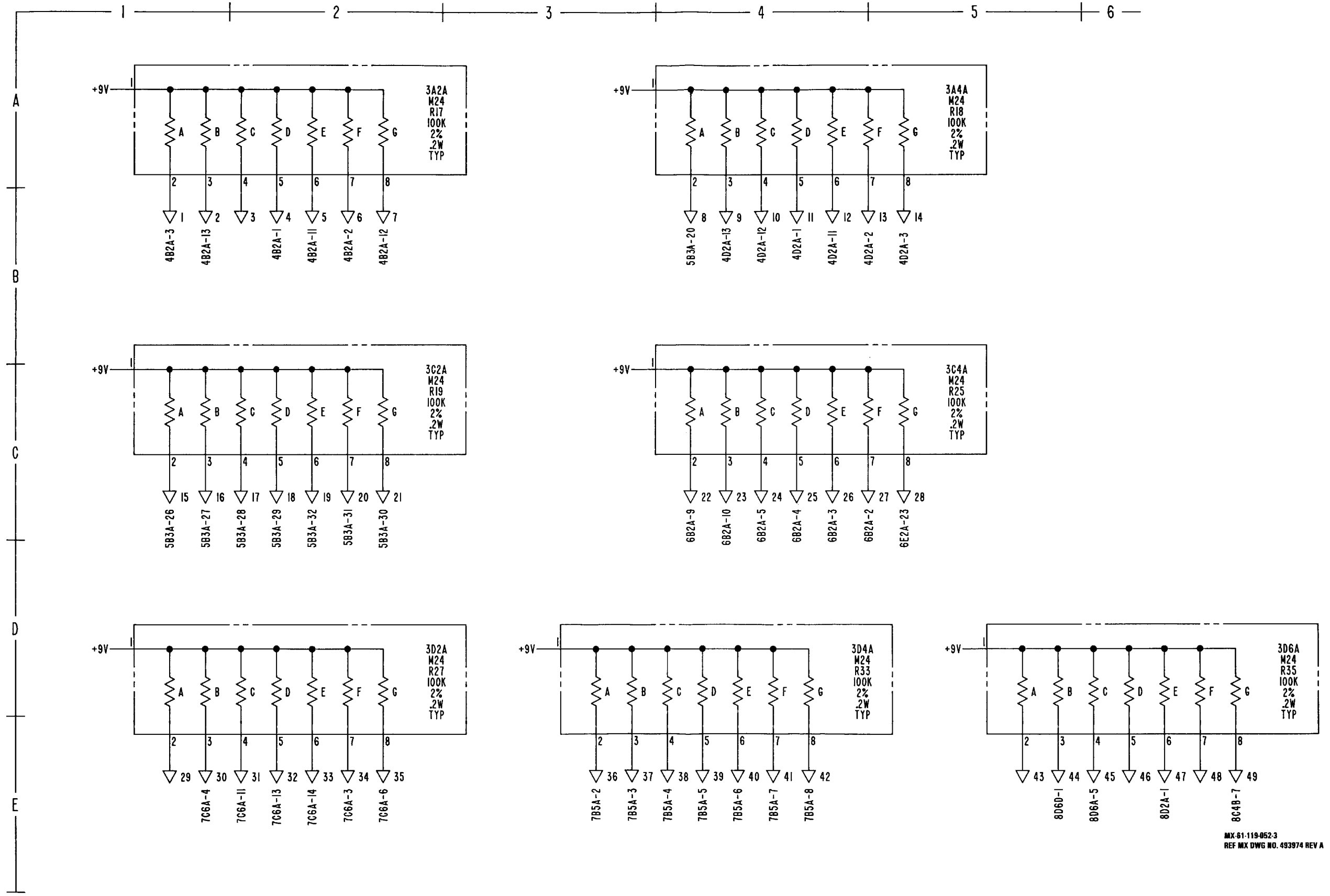
FO-10. RSC Digital Interface Schematic Diagram (Sheet 3 of 12)
