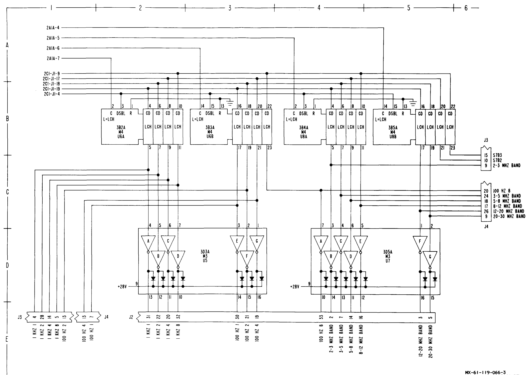
FO-20. RT Interface Schematic Diagram (Sheet 3 of 3)
